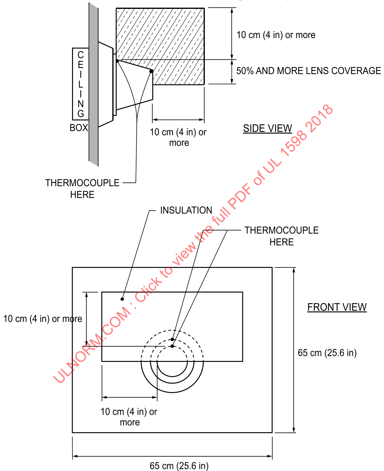
Figure 13.8.2.3 (CAN) Temperature test with luminaire facing horizontally
