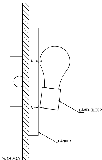
Figure 7.2.3.1 Minimum lamp spacings for wall-mounted luminaries
