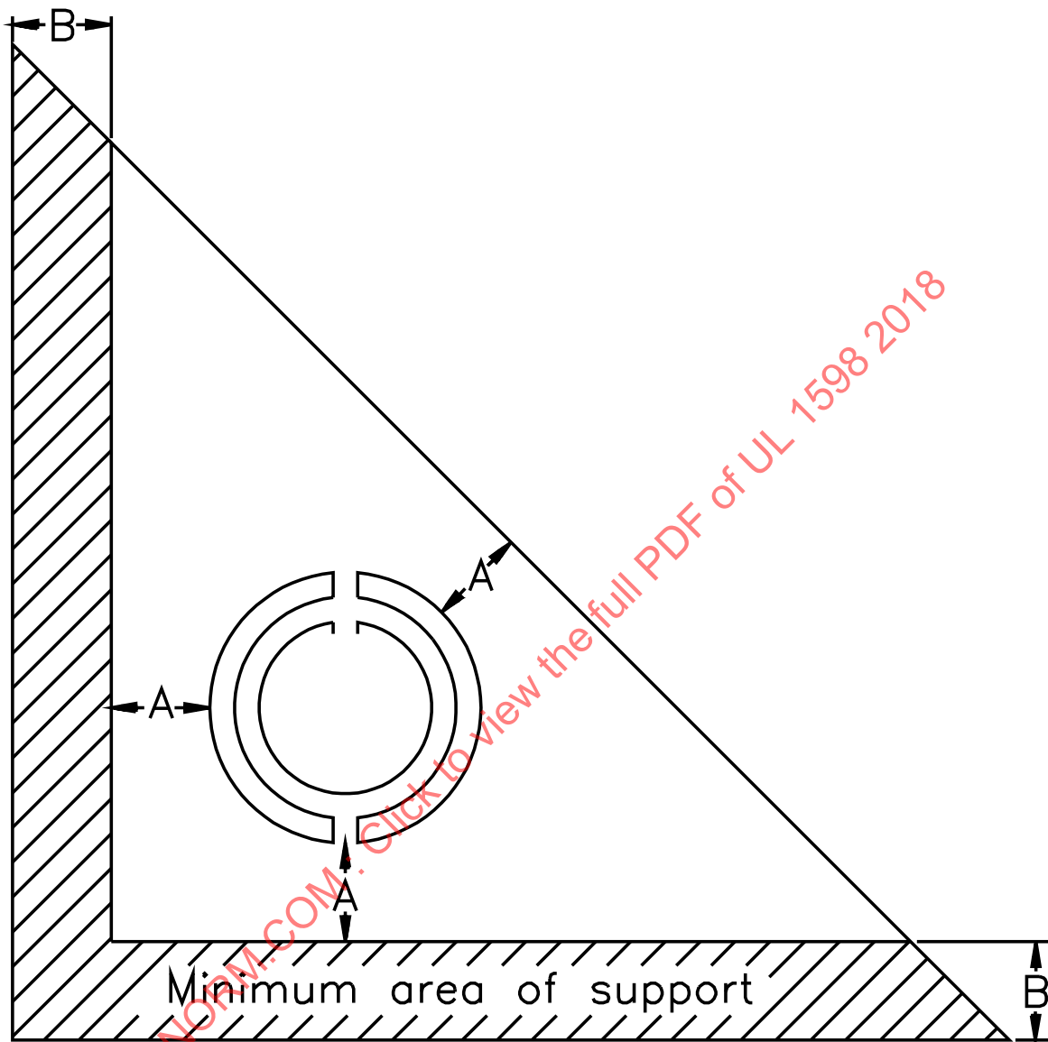
Figure 19.23.1 Knockout and twistout test plate support apparatus (See Clause 19.23.1.)
