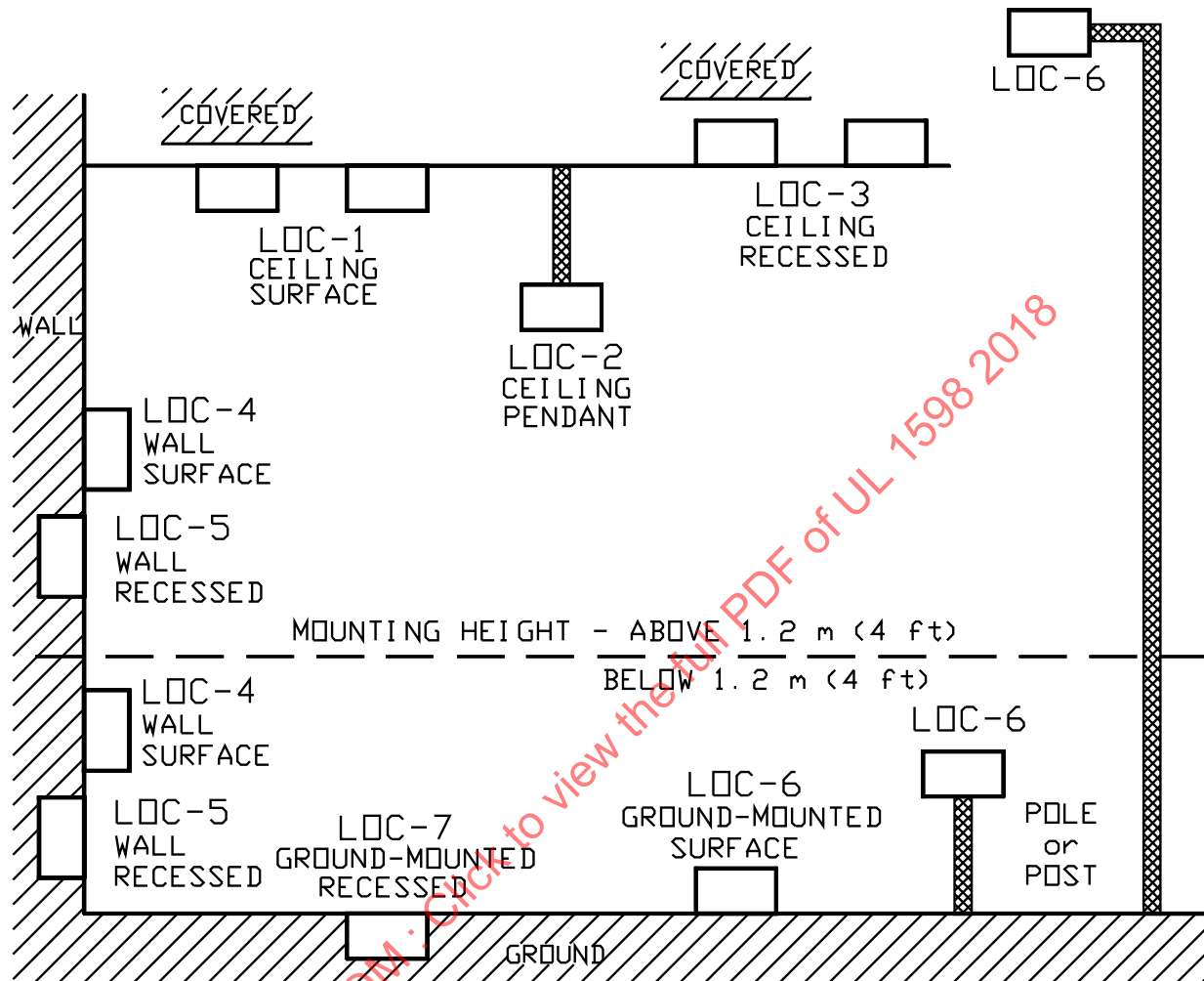
Figure 14.4.8.1 Luminaire location designations
