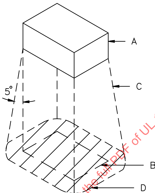
Figure 11.4.1 Location of baffle – directly below (See Clauses 11.4.3, 11.4.4, and 11.4.6.)
