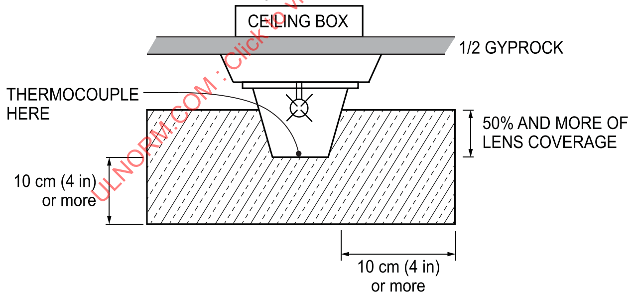
Figure 13.8.2.2 (CAN) Temperature test for TF2
