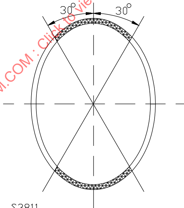
Figure 11.2.1 Chain links
