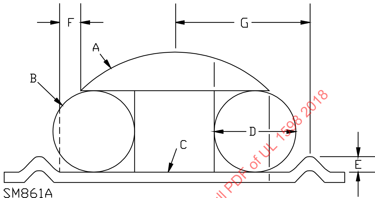
Figure 6.14.2.1 Terminal-conductor relationship
