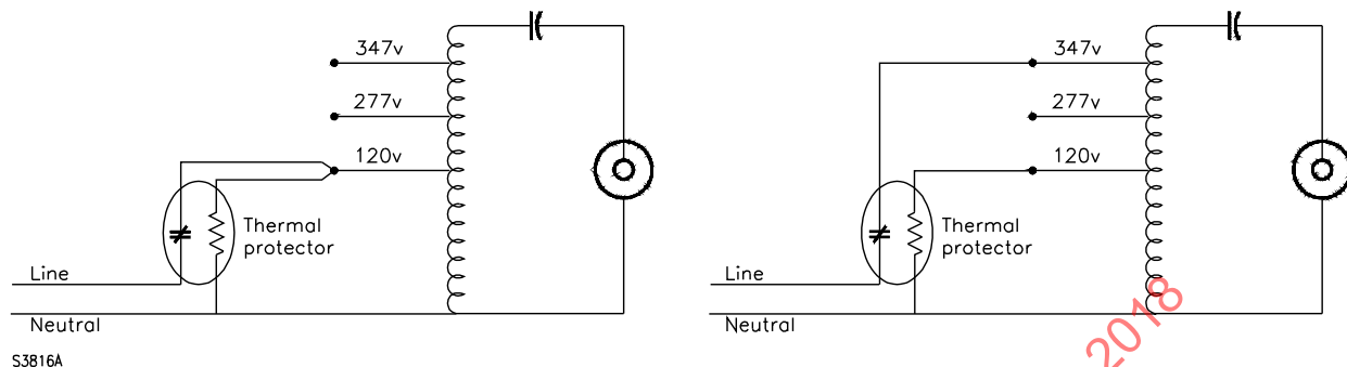
Figure 12.5.1.2 Wiring diagrams for an HID luminaire with a multi-tap autotransformer ballast and thermal protector with a 120 V integral heater
