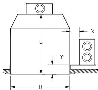
Figure 12.6.1.1 Access to supply connections
