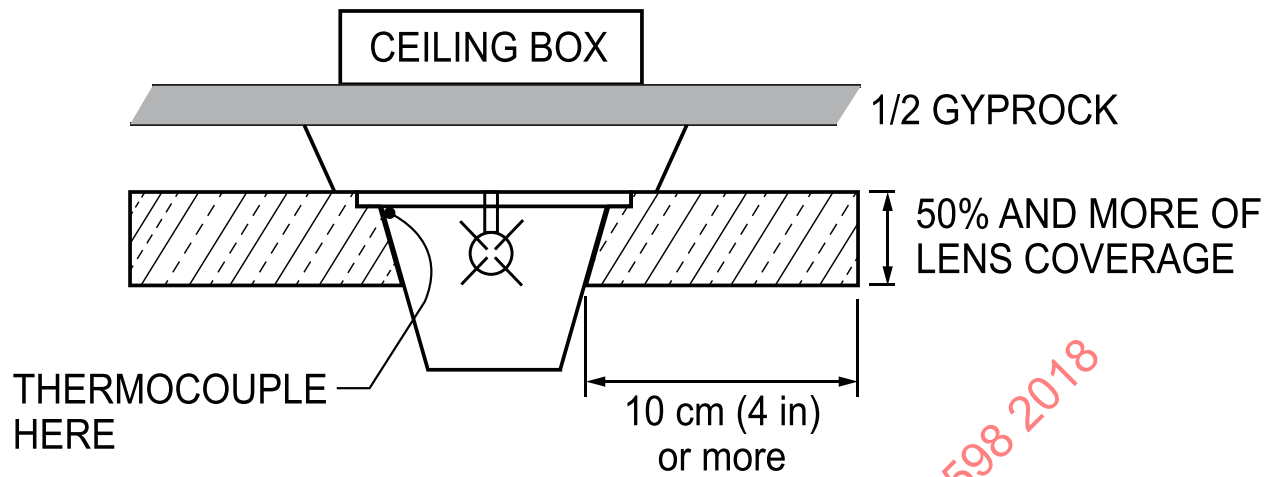
Figure 13.8.2.1 (CAN) Temperature test for TF1
