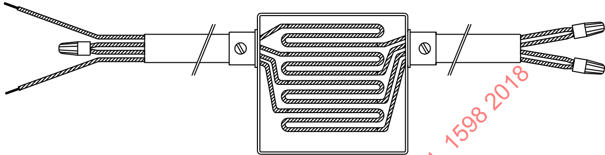
Figure 15.10.1 Test conductor installation for through-wiring junction box temperature test (See Clause 15.10.4.)
