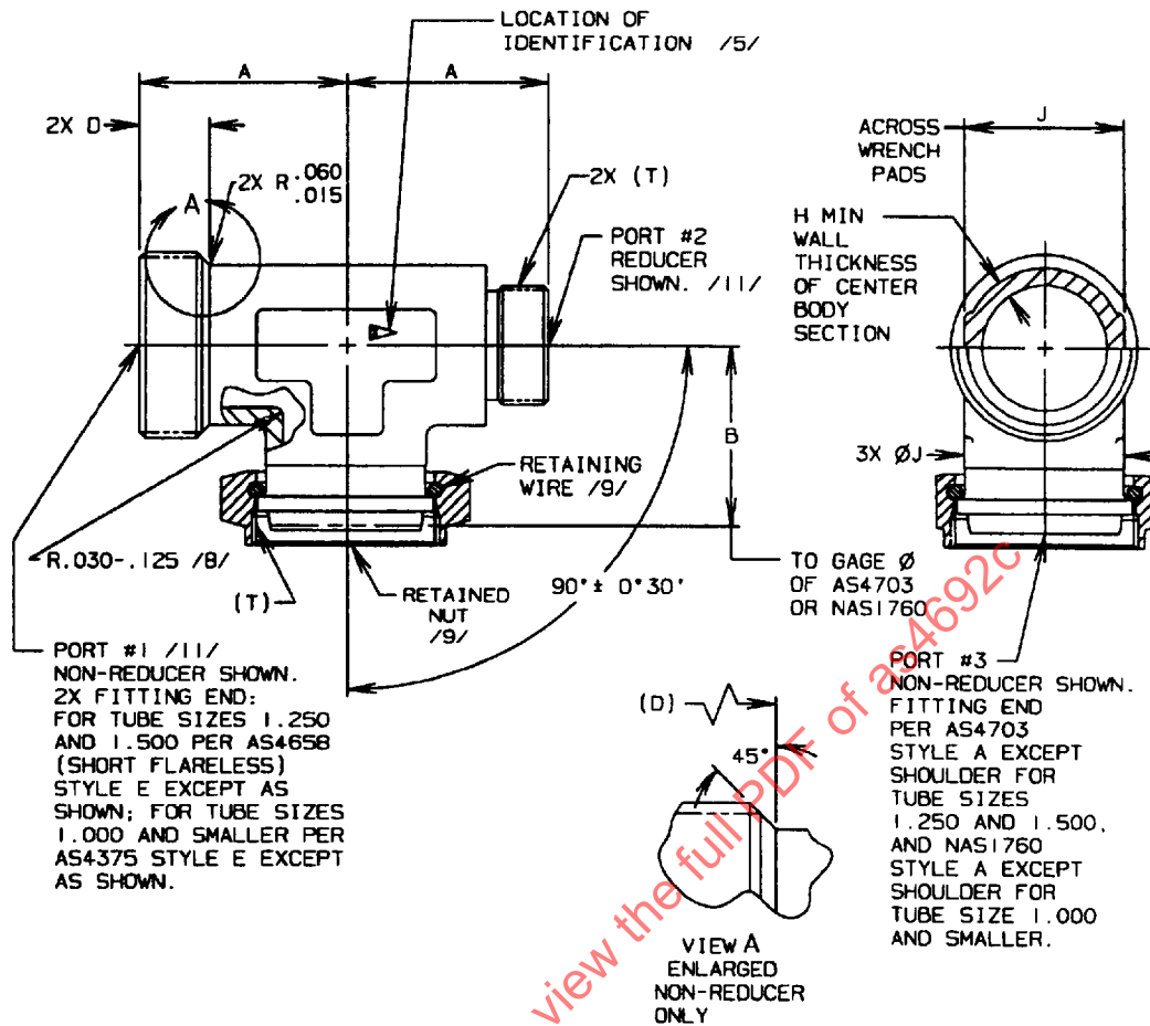
FIGURE 1 - TEE ASSEMBLY
