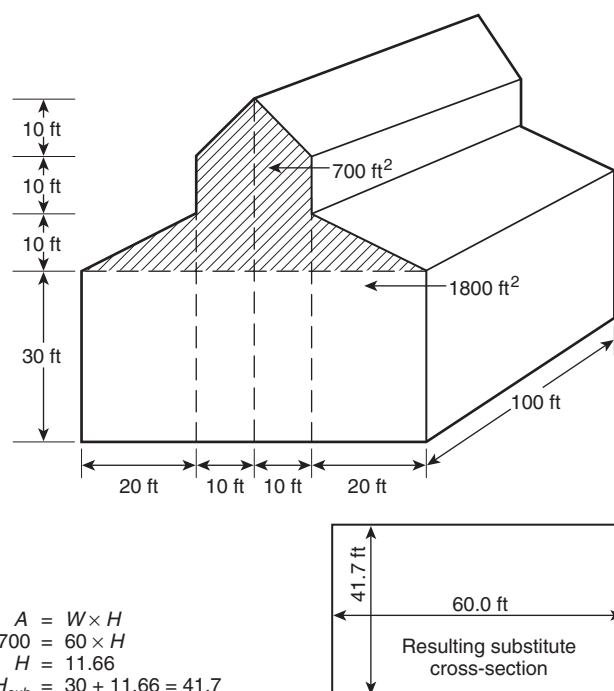
FIGURE C.1.3.1(a) Large Space with Nonflat Ceiling.
