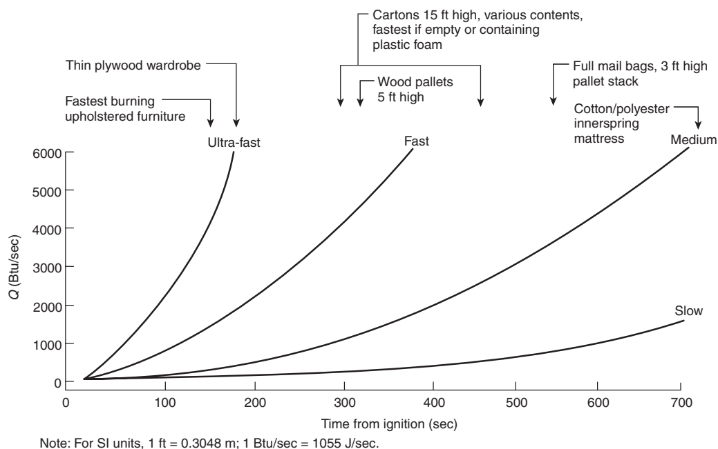
FIGURE B.7.2(c) Relation of t^2 -Squared Fire to Some Fire Tests.
