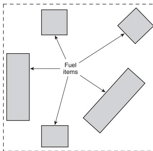
FIGURE A.5.2.5(b) Fuel Items.
