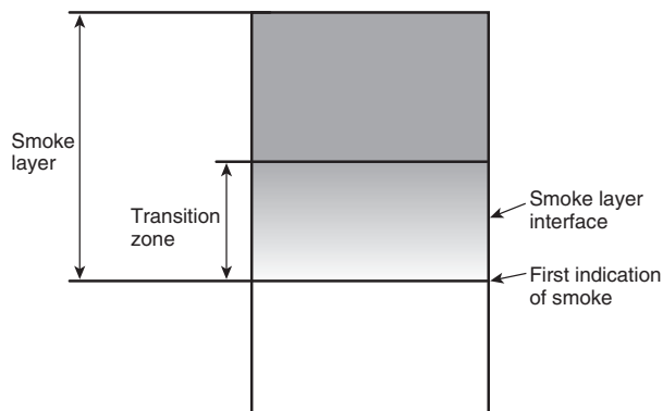
FIGURE A.3.3.13.1 First Indication of Smoke.
