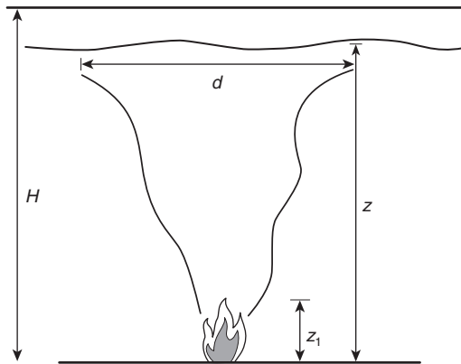
FIGURE A.3.3.11.1 Approximation of an Axisymmetric Plume.
