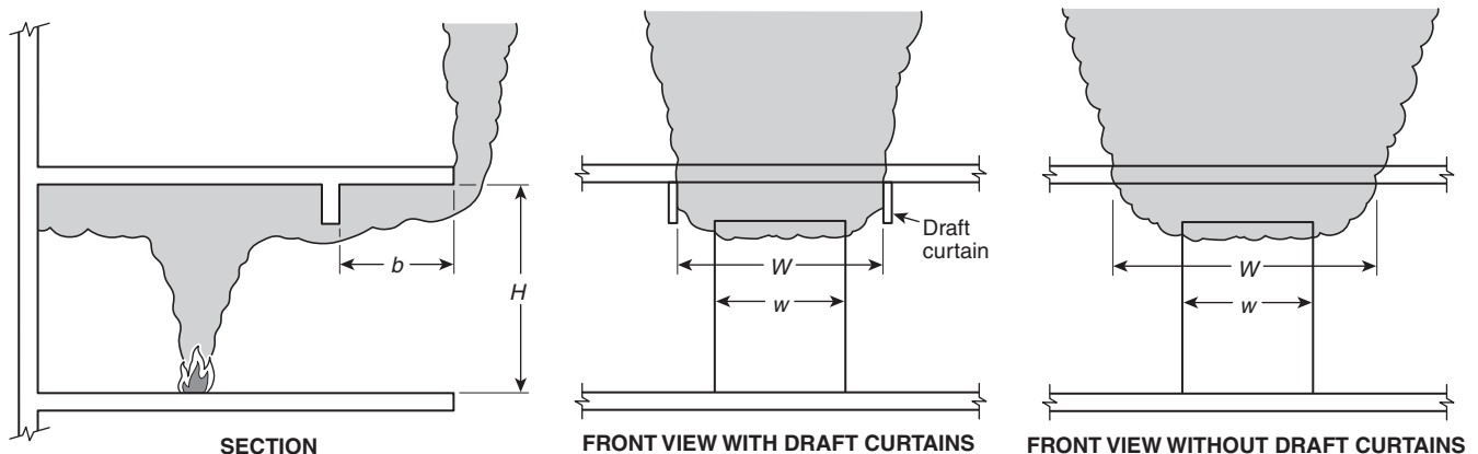
FIGURE A.3.3.11.2 Approximation of a Balcony Spill Plume.
