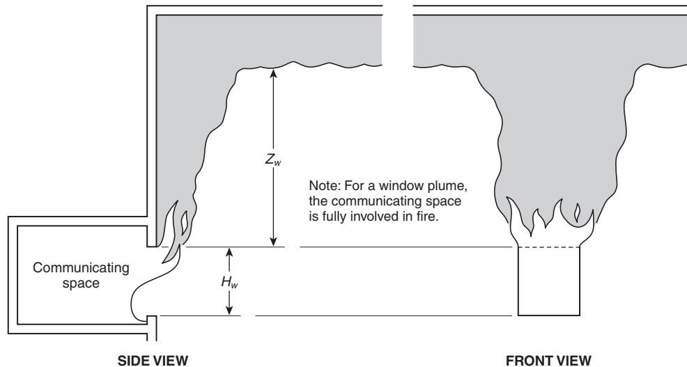
FIGURE A.3.3.11.3 Approximation of a Window Plume.
