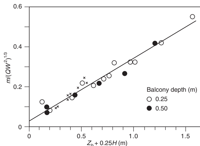
FIGURE A.5.5.2.1 Agreement Between Predictions and Experimental Values (Morgan and Marshall [35]; Mulholland [37]).
