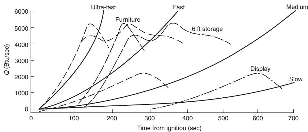
FIGURE B.7.2(b) Rates of Energy Release in a t -Squared Fire. (Source: Nelson [62])
