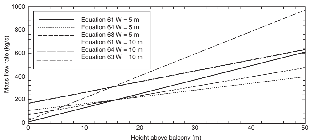
FIGURE A.5.5.2.8 Estimated Mass Flow Rates.
