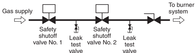
FIGURE A.7.5.15(a) Example of a Gas Piping Diagram for Leak Test. [86:Figure A.7.4.9(a)]
