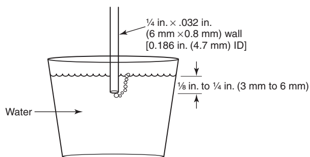
FIGURE A.7.5.15(c) Leak Test for a Safety Shutoff Valve. [86:Figure A.7.4.9(c)]
