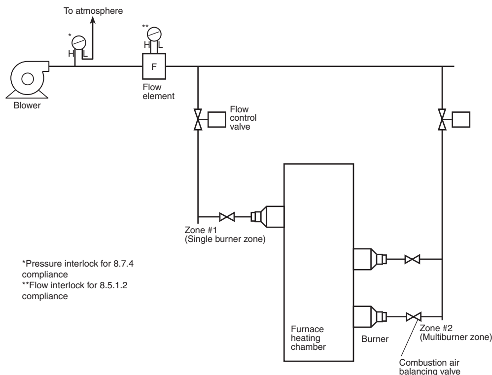
FIGURE A.8.7.4 Examples of Air Proving Devices Used in Multiburner Systems (fuel piping not shown for clarity).
