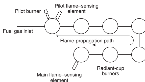
FIGURE A.8.10.6(b) Example of a Combustion Safeguard Supervising a Group of Radiant Cup Burners Having Reliable Flame-Propagation Characteristics from One to the Other by Means of Flame-Propagation Devices.
