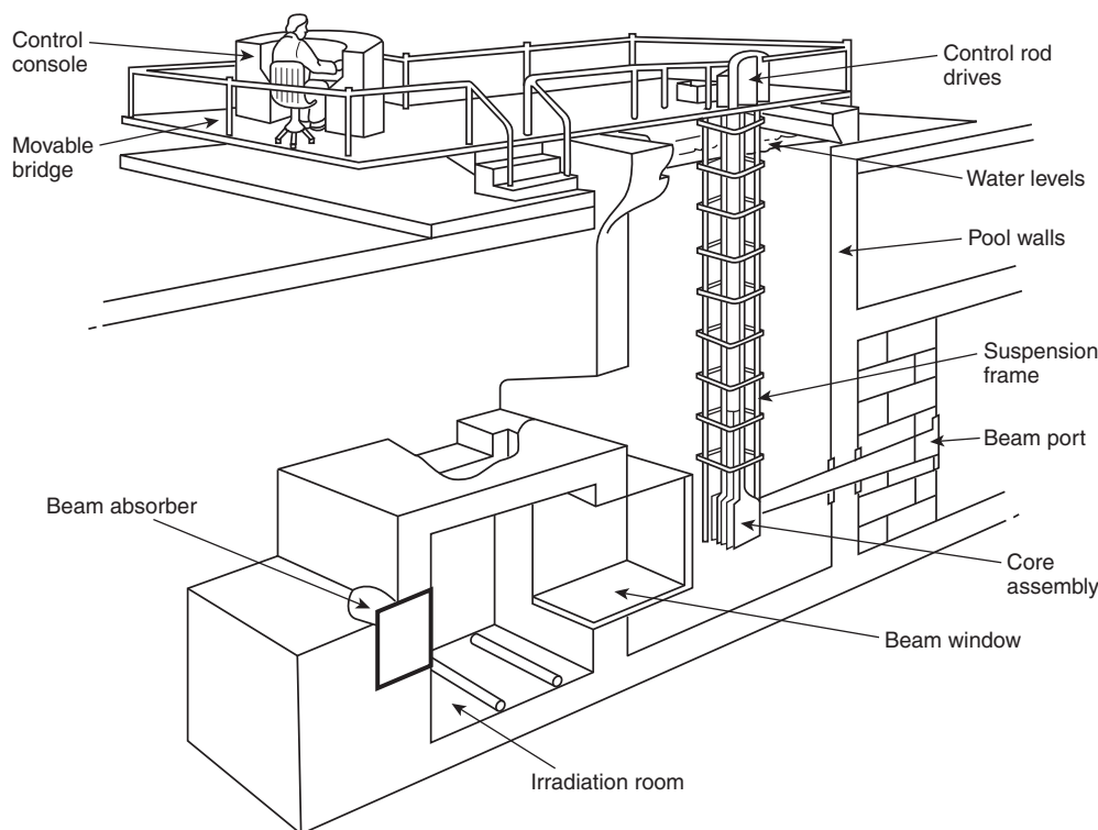
FIGURE B.11.2 Open Pool (Swimming Pool) Reactor Assembly.
