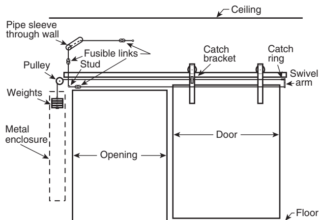
FIGURE A.4.7.5(e) Closing Devices for Single Sliding Door, Example 2 (Level Track).
