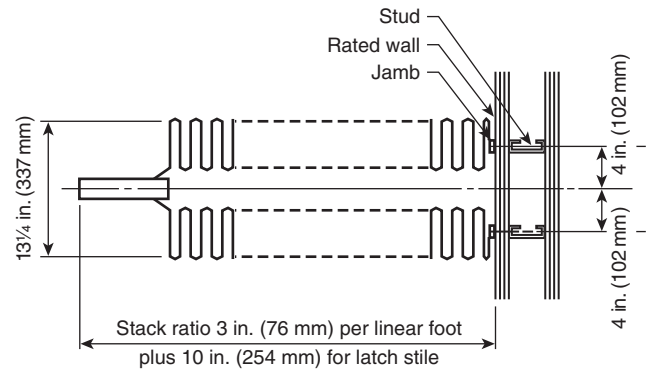
FIGURE A.9.1.3(b) Typical Horizontally Sliding Accordion or Folding Door with No Pocket.
