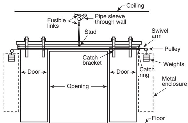
FIGURE A.4.7.5(h) Closing Devices for Center-Parting, Horizontally Sliding Doors, Example 2 (Level Track).
