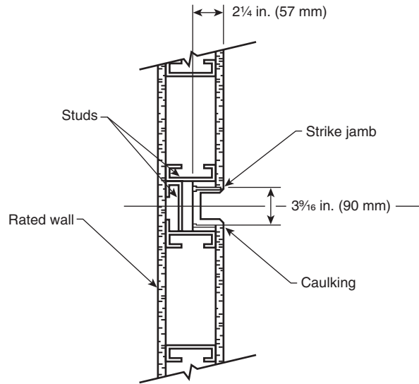
FIGURE A.9.1.3(a) Typical Strike Jamb for Horizontally Sliding Accordion or Folding Door.
