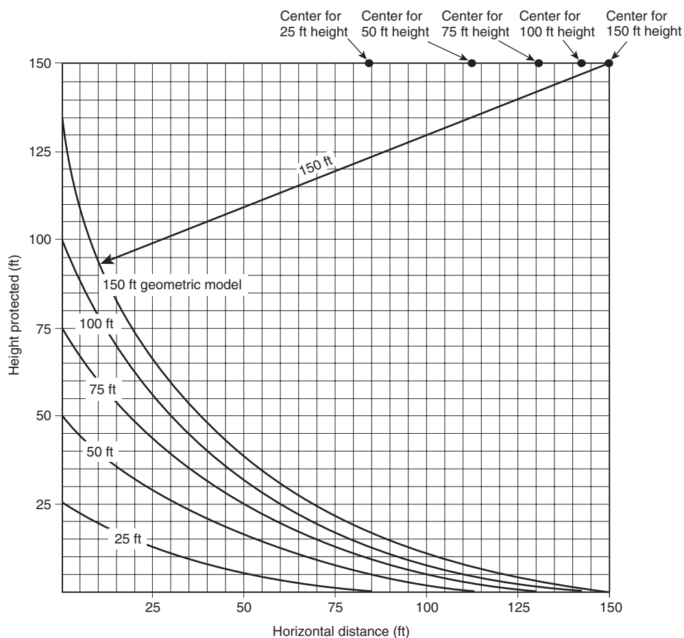
FIGURE 4.7.3.3 Zone of Protection Utilizing Geometric Model.
