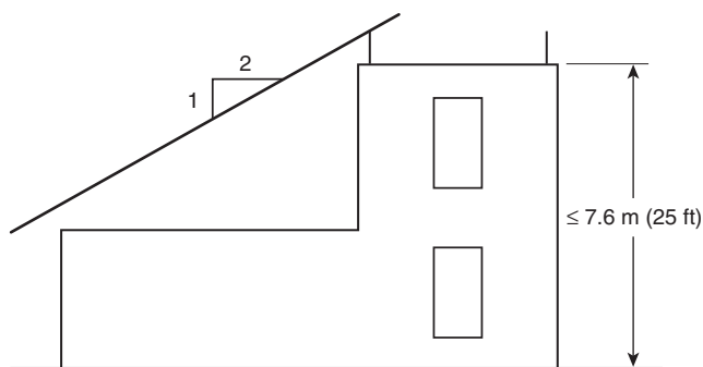
FIGURE 4.7.2.3(a) Lower Roof Protection for Flat Roof Buildings 7.6 m (25 ft) or Less in Height.
