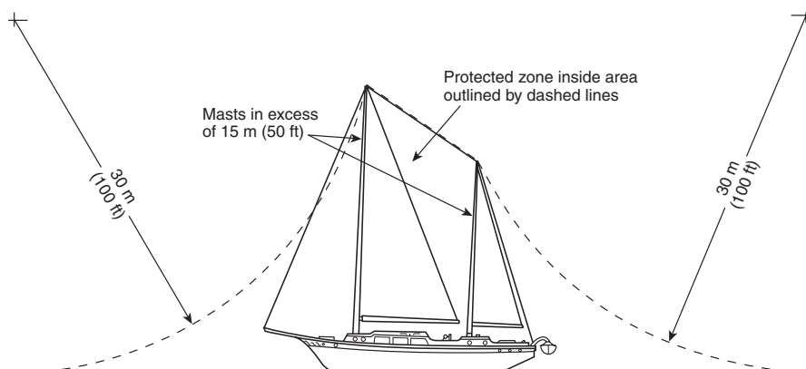
FIGURE 8.3.1.2(b) Diagram of Boat with Masts in Excess of 15 m (50 ft) Above the Water; Protection Based on Lightning Strike Distance of 30 m (100 ft).
