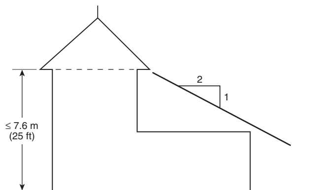
FIGURE 4.7.2.3(b) Lower Roof Protection Provided by Pitched Roof Buildings 7.6 m (25 ft) or Less in Height.
