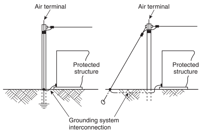
FIGURE 7.3.3.9 Alternate Grounding Methods for Overhead Ground-Wire Protection.
