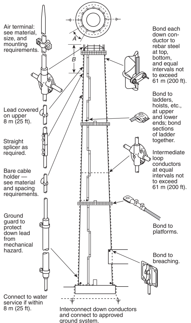
FIGURE 6.1 Heavy-Duty Stack.
