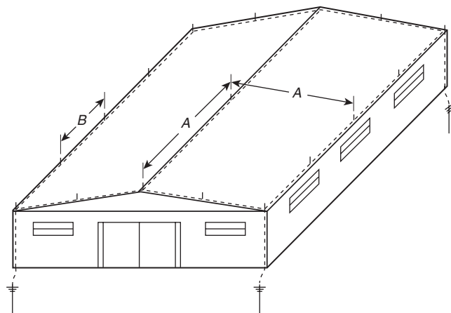
FIGURE 4.8.2.4(a) Air Terminals on Flat Roof.
