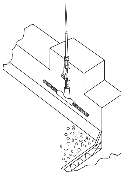
FIGURE 4.8.5.5 Irregular Roof Perimeter.
