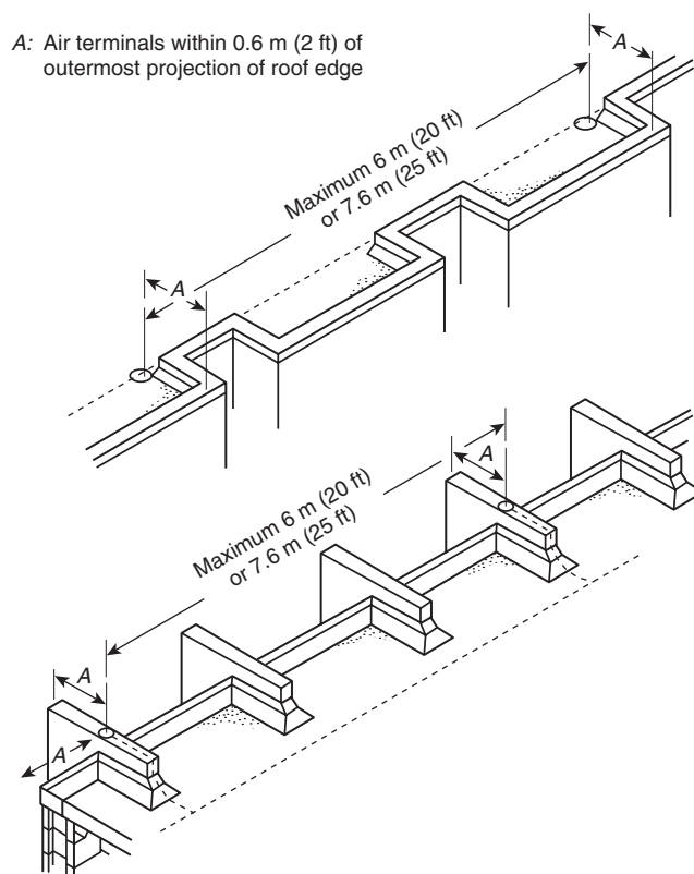
FIGURE 4.8.5.2 Flat or Gently Sloping Roof with Irregular Perimeter.
