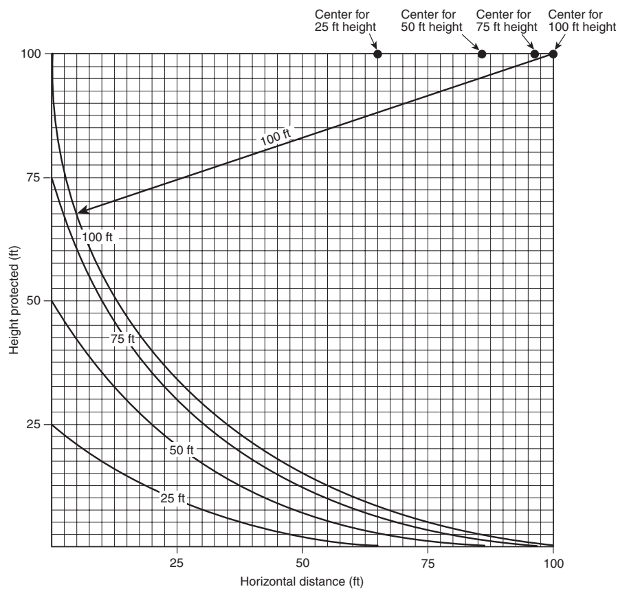
FIGURE 7.3.3.2 Single Mast Zone of Protection (a) and Overhead Ground Wires Zone of Protection (b).
