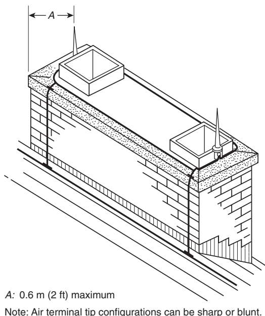
FIGURE 4.8.8.3 Air Terminals on Chimney.
