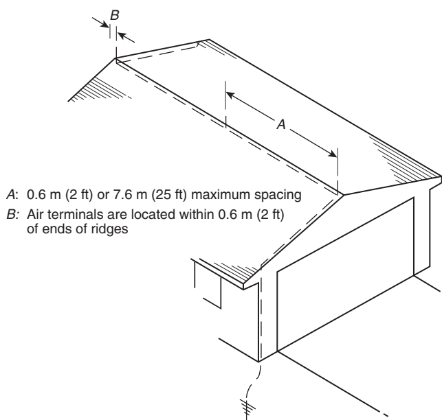
FIGURE 4.8.2 Air Terminals on Pitched Roof.
