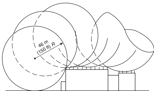
FIGURE 4.7.3.1(B) Zone of Protection Depicting Rolling Sphere.
