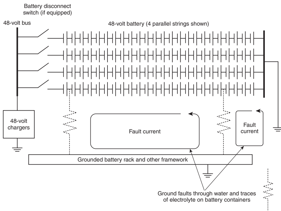
FIGURE A.8.6.2.2.1 Battery Ground Fault Path Through Spilled or Sprinklered Water or Mist.
