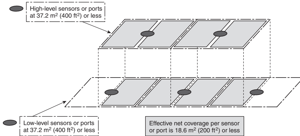
FIGURE A.8.5.3.1.2.2 Staggered Layout of Sample Ports/Sensors.
