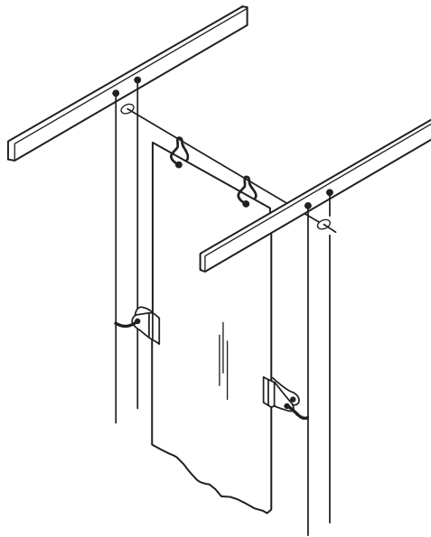
FIGURE 13.1.3 Test Sample Flat Sheet.
