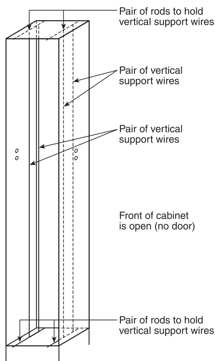
FIGURE 12.2.1.2.3.2 Vertical Guide Support.
