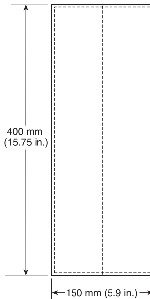
FIGURE 7.1.4 Multilayer Specimen for Test Method 1.
