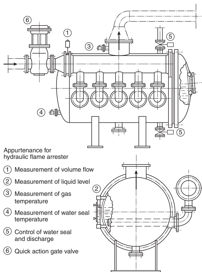
FIGURE A.12.2.6.1(b) Sparge Tube Hydraulic Arrester.
