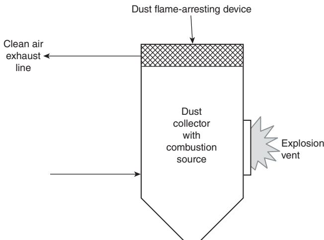
N FIGURE A.12.2.8(b) Typical Application of Dust Flame-Arresting Device Integrated into Clean Air Plenum.
