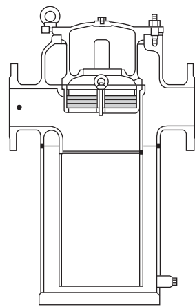
FIGURE A.12.2.7.1(a) Liquid Product Detonation Arrester with Siphon Bypass (Emptying and Filling Lines).
