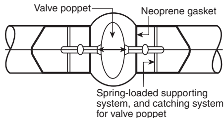
FIGURE A.12.2.2.1 Flow-Actuated Float Valve.
