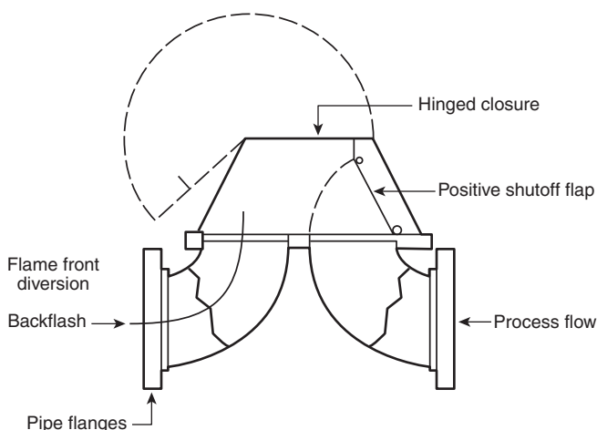
FIGURE A.12.2.1.1(b) Explosion Door Diverter.
