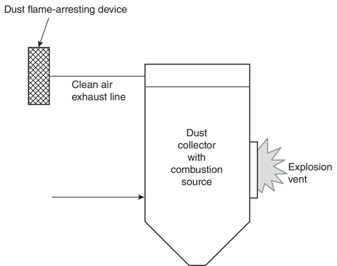
N FIGURE A.12.2.8(c) Typical End-of-Line Application of Dust Flame-Arresting Device.
