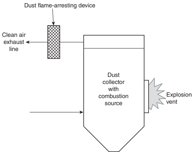
N FIGURE A.12.2.8(a) Typical Application of Dust Flame-Arresting Device.
