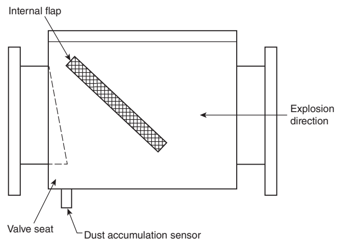
FIGURE A.12.2.3.4.5 Example of Dust Accumulation Sensor on a Flow-Actuated Flap Valve.
