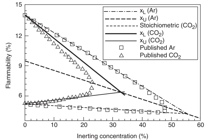
FIGURE B.7.3 Methane with Argon or CO 2 Diluent [Ma (2011), Figure 5(a)].
