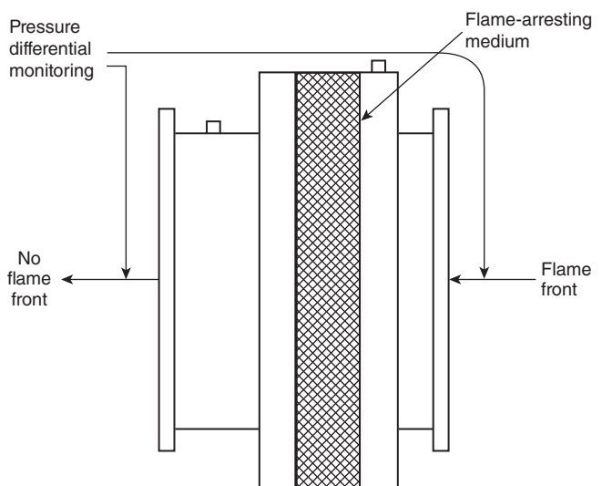
N FIGURE A.12.2.8(d) Dust Flame-Arresting Device.
