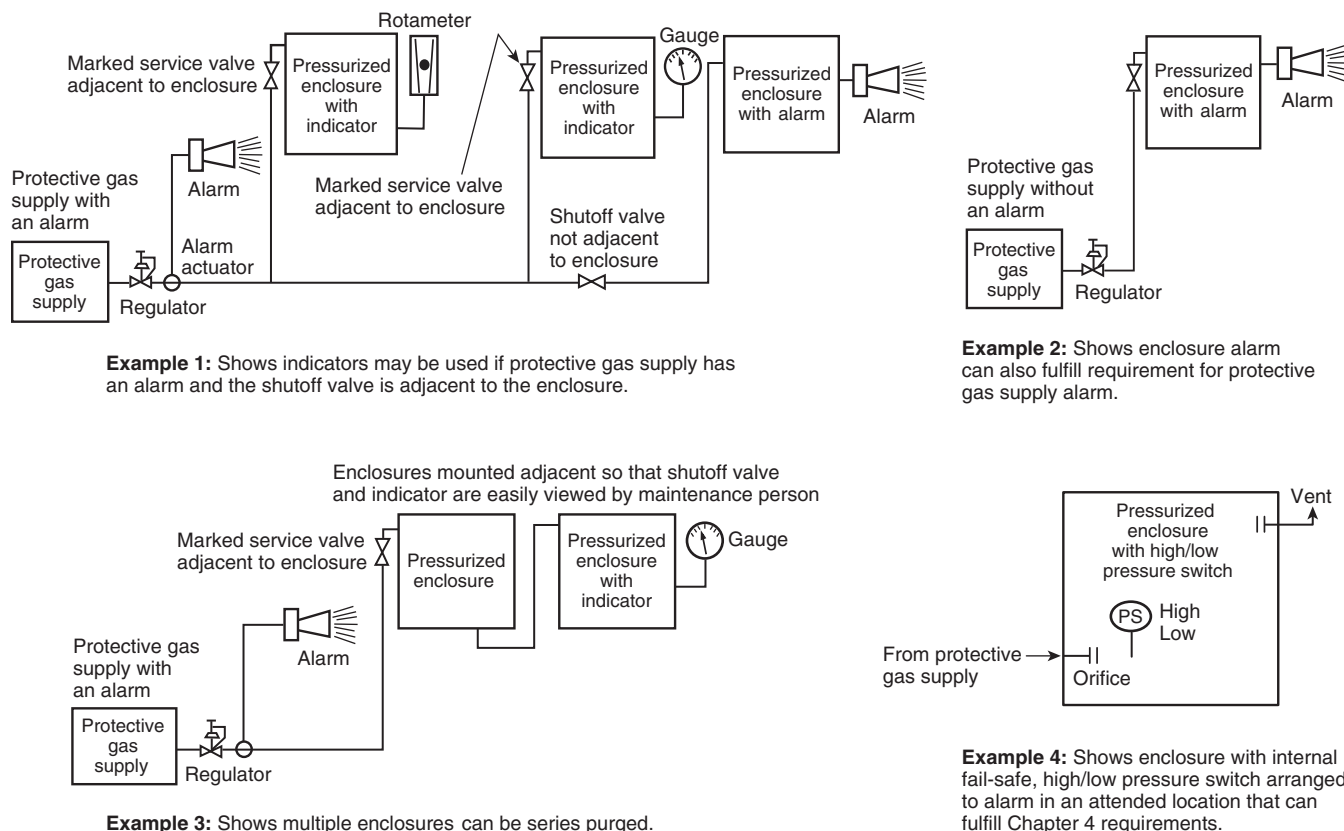
FIGURE A.4.9 Typical Alarm and Indicator Configurations for Types Y and Z Pressurizing. Purge outlet devices that could be provided are not shown for clarity.
