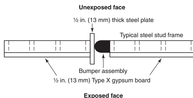
FIGURE A.6.4.9.1 Proposed Method for Testing of Bumper Assemblies.
