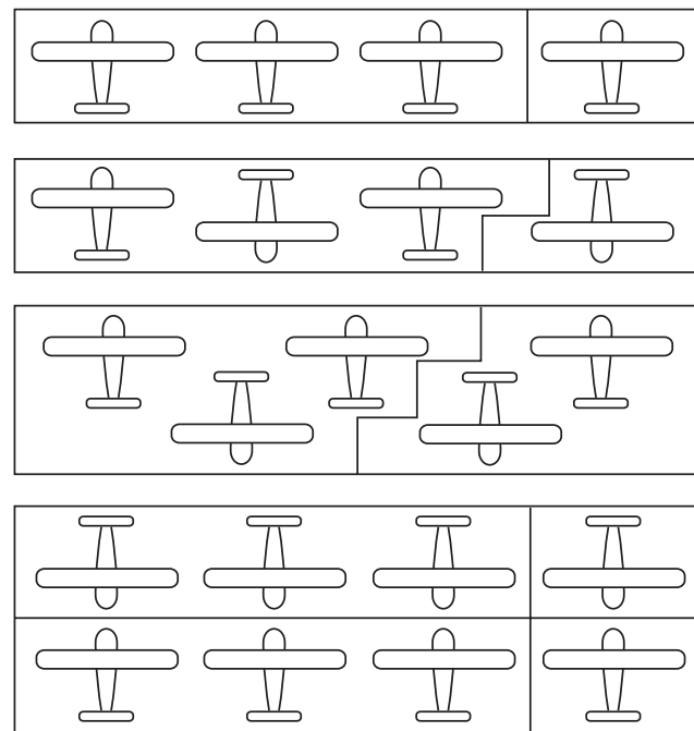
Figure A-1-3(b) Typical configurations of row hangars.
