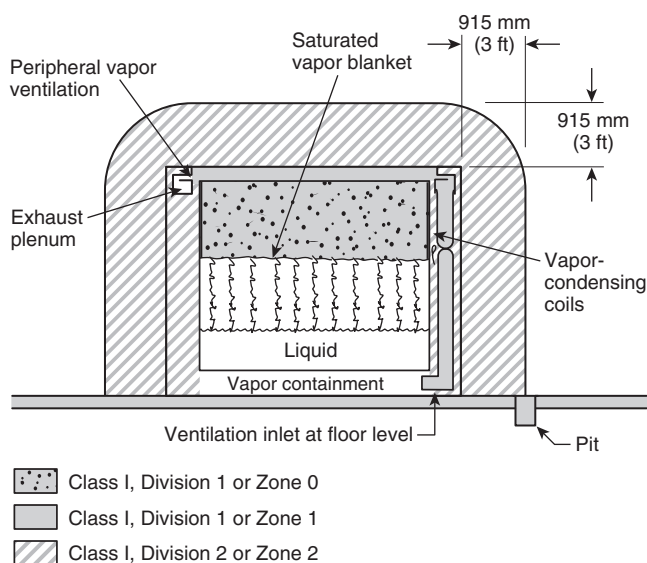
FIGURE 6.4(d) Electrical Area Classification for Open Dipping and Coating Process with Partial Peripheral Vapor Containment and Ventilation — Vapors Confined to Process Equipment.
