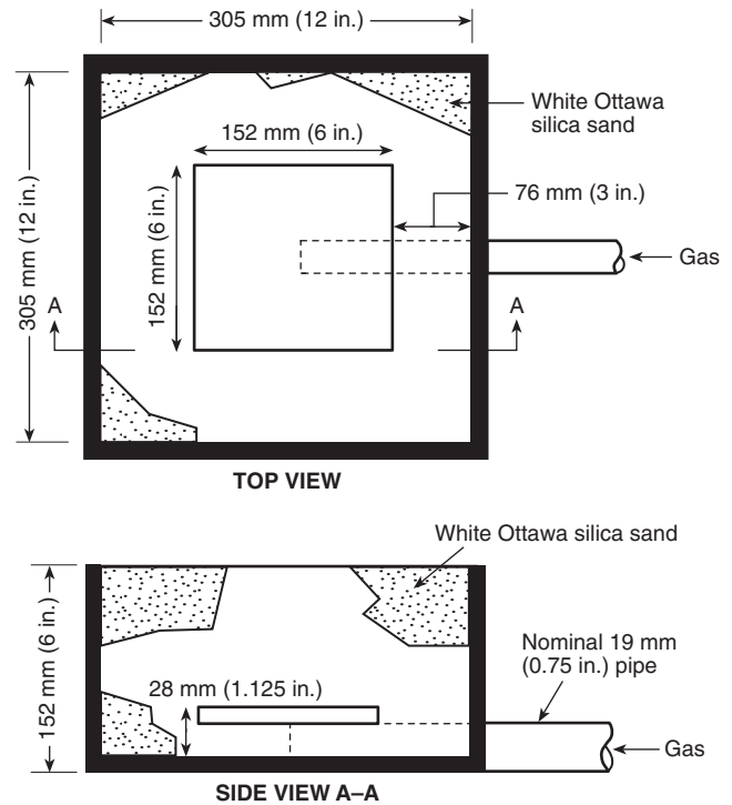
FIGURE 4.1.1 Gas Burner.
