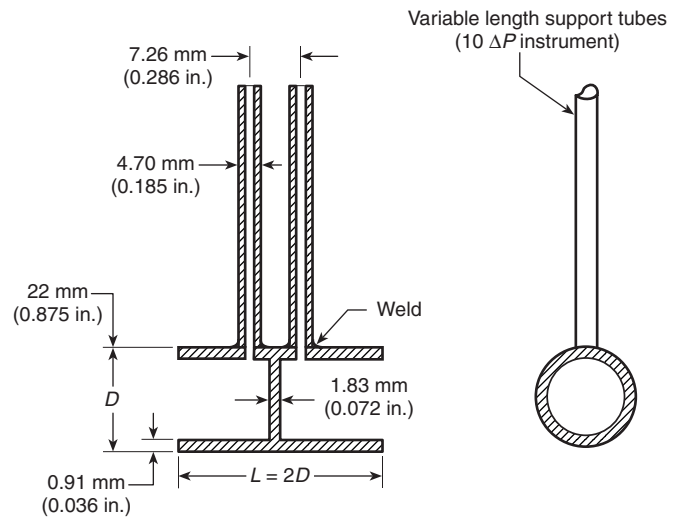
FIGURE 7.3.2.1 Bidirectional Probe.
