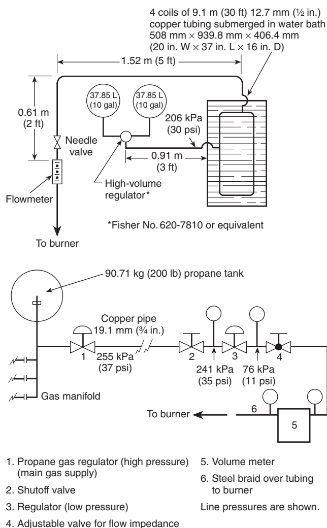
FIGURE A.4.1.6 Two Typical Gas Flow Regulation Systems.
