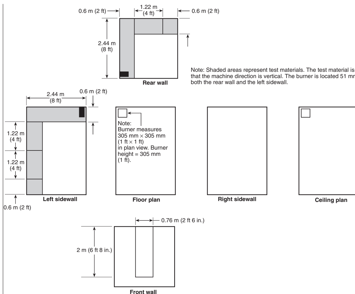
FIGURE C.2.1 Specimen Mounting for Method A Test Protocol.
