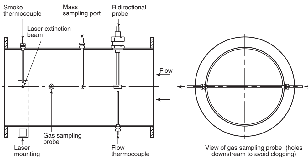
FIGURE 7.3.8.3.2(b) Recommendations for Mounting the Laser Beam and Other Instrumentation in Exhaust Duct.
