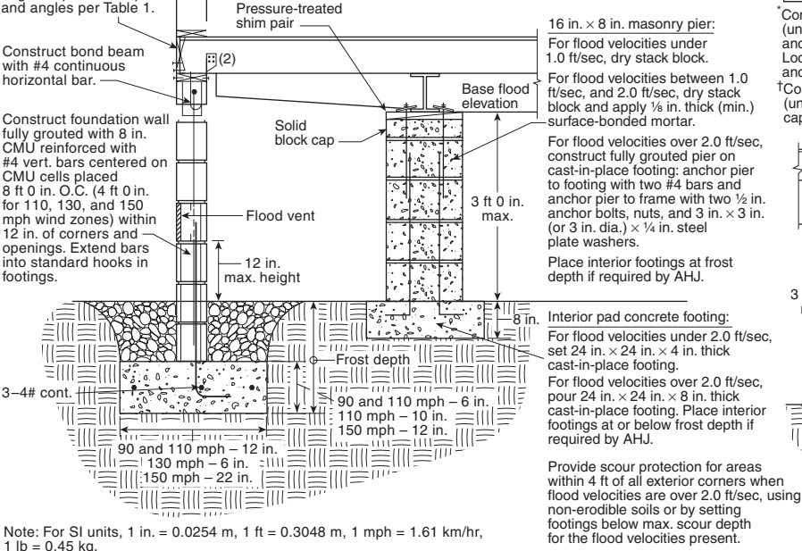
FIGURE 15.5.1.1(b) Masonry/Concrete Foundation Longitudinal Wall and Pier Details.
