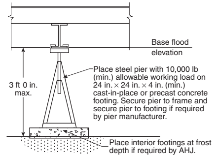
Steel Pier Alternate for Flood Velocities Under 1 ft/sec
