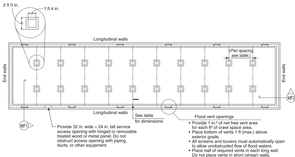
FIGURE 15.5.2.2(a) Masonry/Concrete Foundation Plan — Single Unit.
