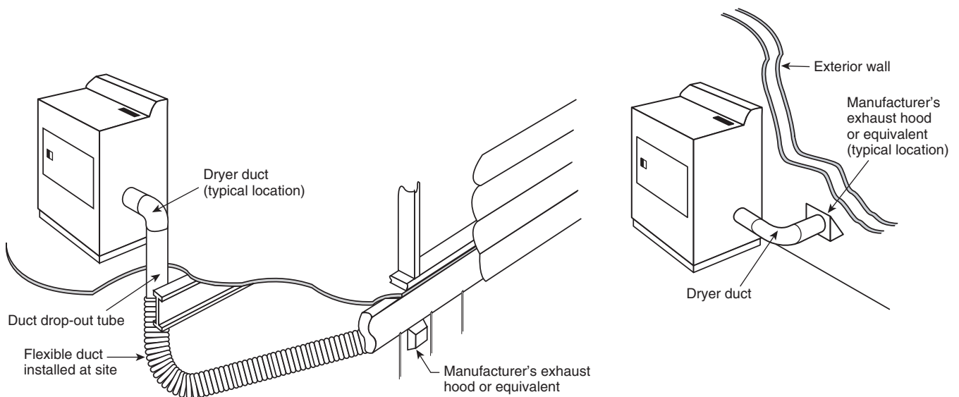
FIGURE 8.7(c) Installation of Field-Applied Horizontal Lap Siding.
