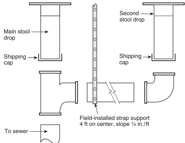
FIGURE 10.3.2.1 Drain Pipe Slope and Connections.
