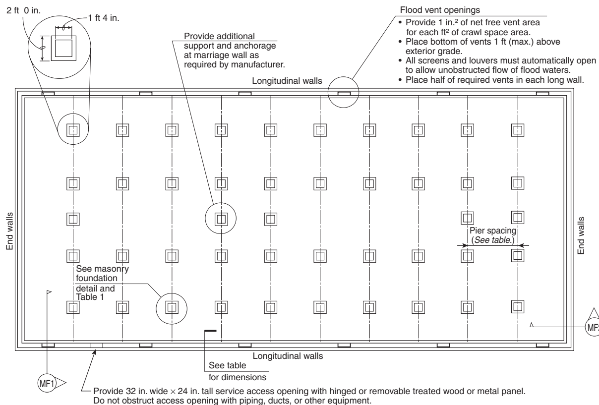
FIGURE 15.5.2.2(b) Masonry/Concrete Foundation Plan — Double Unit.
