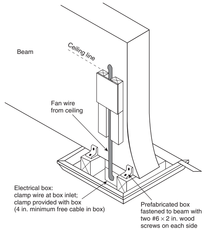
FIGURE 8.5.6.2(a) Electrical Outlet Box and Support Structure for Ceiling-Suspended (Paddle) Fan.
