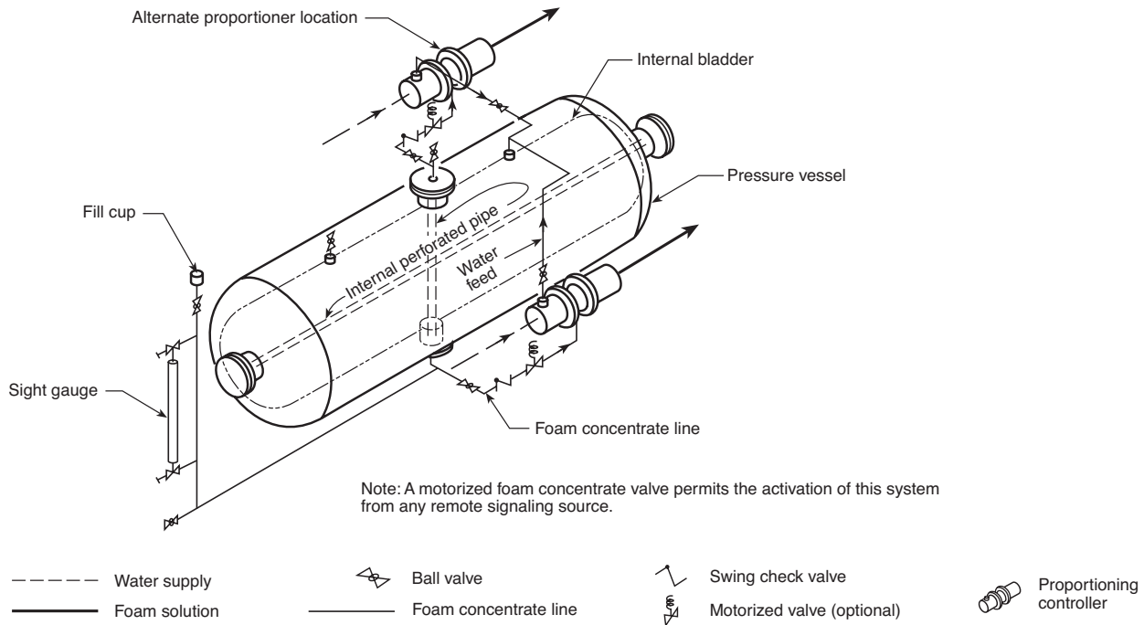
FIGURE A.5.4.2(e) Balanced-Pressure Proportioning (Bladder System).
