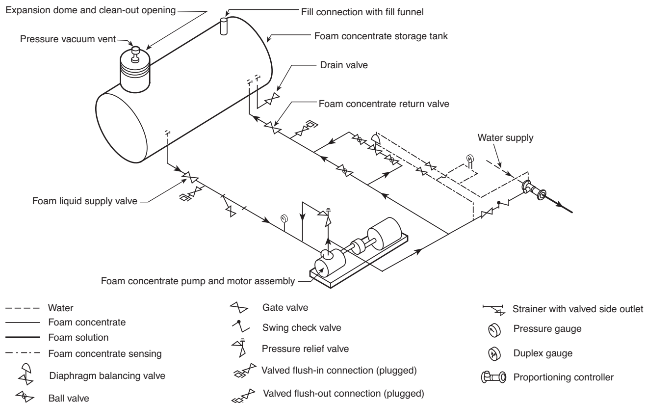
FIGURE A.5.4.2(d) Balanced-Pressure Proportioners (with Concentrate Pump).
