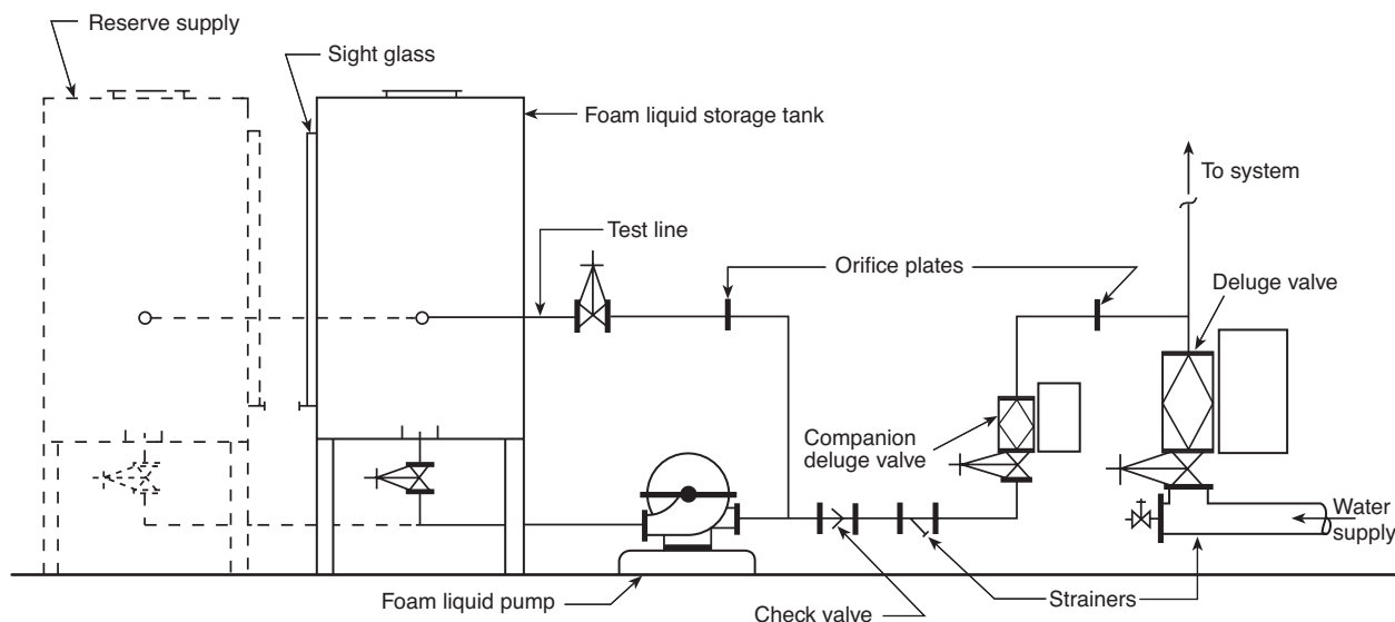
FIGURE A.5.4.2(a) Foam Liquid-Concentrate Storage Tank, Liquid-Concentrate Pump, Metering Proportioners, and Interconnecting Piping.
