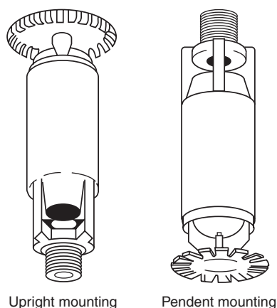
FIGURE A.3.3.6.1 Variations in Deflector Shape.
