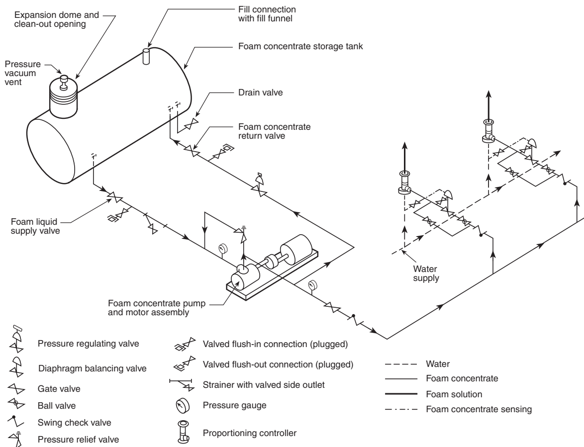
FIGURE A.5.4.2(f) In-Line Balanced-Pressure Proportioning System.
