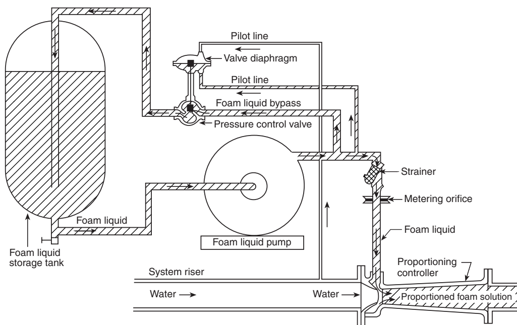
FIGURE A.5.4.2(b) Balanced-Pressure Proportioning System.
