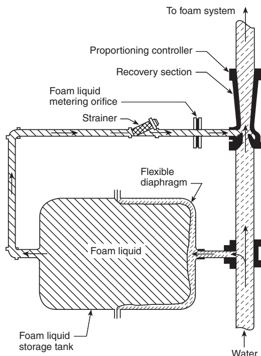
FIGURE A.5.4.2(h) Pressure Proportioning Tank with Diaphragm.
