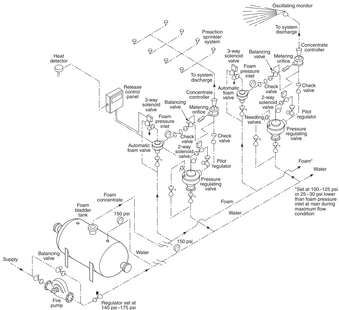
FIGURE A.5.4.2(g) In-Line Balanced-Pressure Proportioning System with Bladder Tank.
