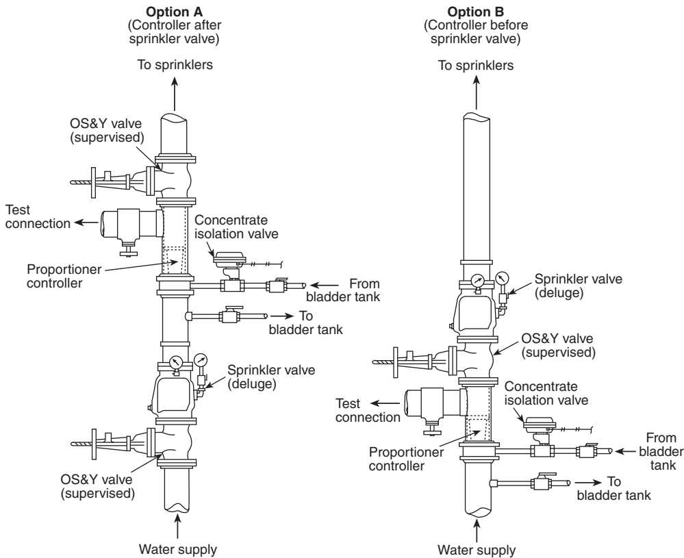
FIGURE A.5.14 Test Connection Detail.
