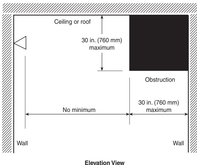
FIGURE 8.2.5.4.2(c) Positioning of Sprinkler to Avoid Obstructions Against Wall (Residential Sidewall Sprinklers).
