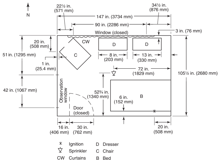
FIGURE A.1.1(b) Manufactured Home Bedroom.
