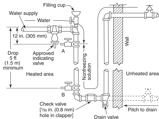
FIGURE 9.2.3.2.1 Arrangement of Supply Piping with Backflow Device.
