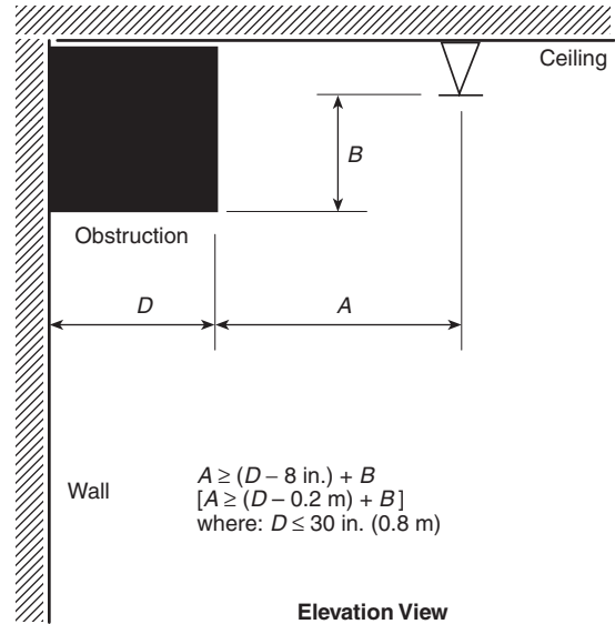
FIGURE 8.2.5.4.3 Positioning of Sprinkler to Avoid Obstruction Against Walls (Residential Upright and Pendent Spray Sprinklers).
