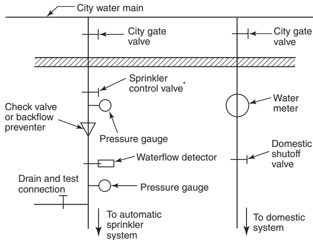
FIGURE A.6.2(b) Acceptable Arrangement for Stand-Alone Piping Systems with Valve Supervision — Option 1.
