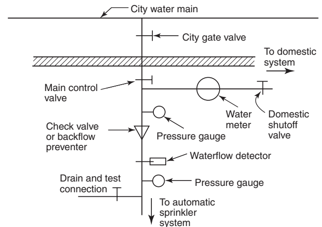
FIGURE A.6.2(a) Preferred Arrangement for Stand-Alone Piping Systems.
