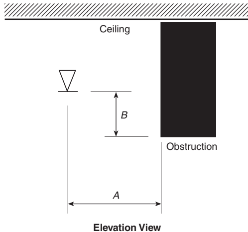
FIGURE 8.2.5.4.2 Positioning of Sprinkler to Avoid Obstruction to Discharge (Residential Upright and Pendent Spray Sprinklers).
