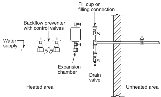
FIGURE 9.2.3.2.1 Arrangement of Supply Piping with Backflow Device.
