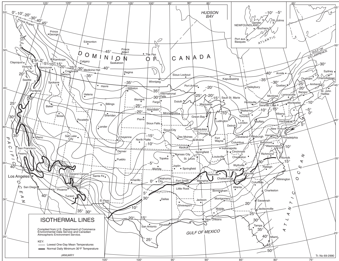
FIGURE A.8.2.6(c) Isothermal Lines — Lowest One-Day Mean Temperature (°F). [24:Figure A.10.5.1]
