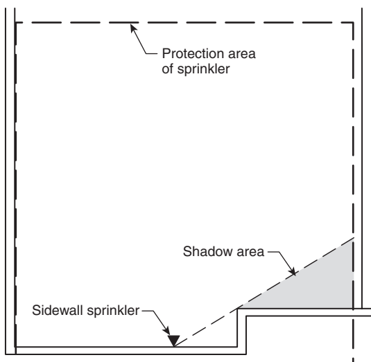
FIGURE A.8.2.5.7(b) Example of Shadow Areas (HSW).
