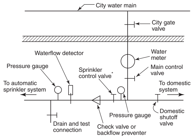
FIGURE A.6.2(c) Acceptable Arrangement for Stand-Alone Piping Systems with Valve Supervision — Option 2.
