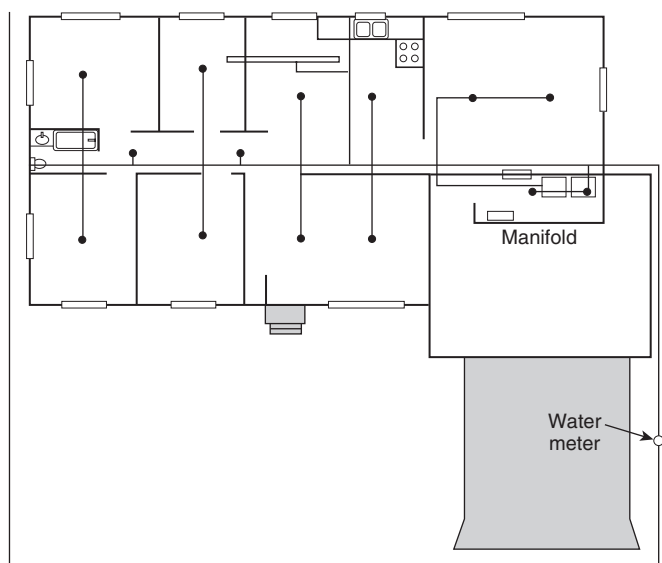
FIGURE A.3.3.9.3(a) Multipurpose Piping System — Example 1.
