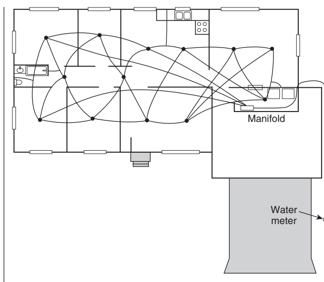
FIGURE A.3.3.9.4 Network System.
