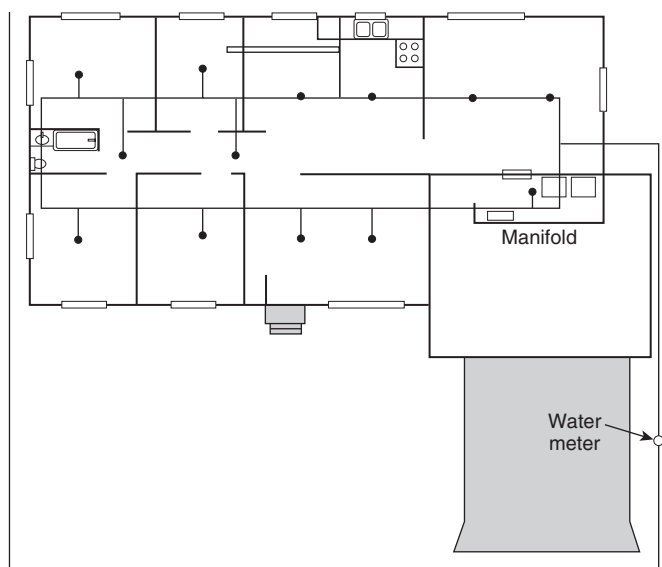
FIGURE A.6.3(b) Multipurpose Piping System — Example 2.
