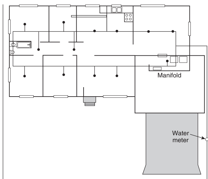
FIGURE A.3.3.9.3(b) Multipurpose Piping System — Example 2.
