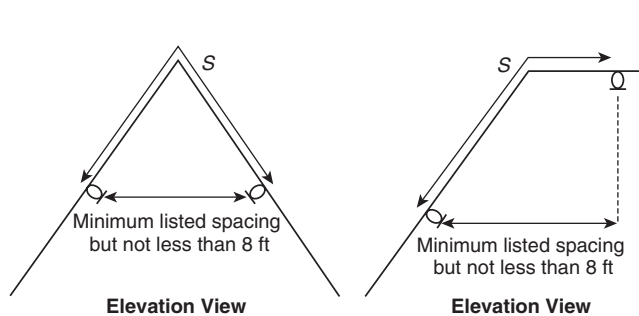
FIGURE 8.1.3.1.3.1 Measuring S Dimension.
