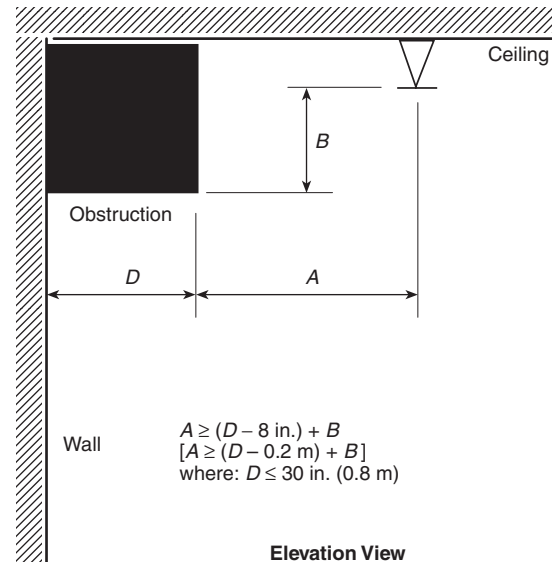
FIGURE 8.2.5.4.3 Obstructions Against Walls (Residential Upright and Pendent Spray Sprinklers).
