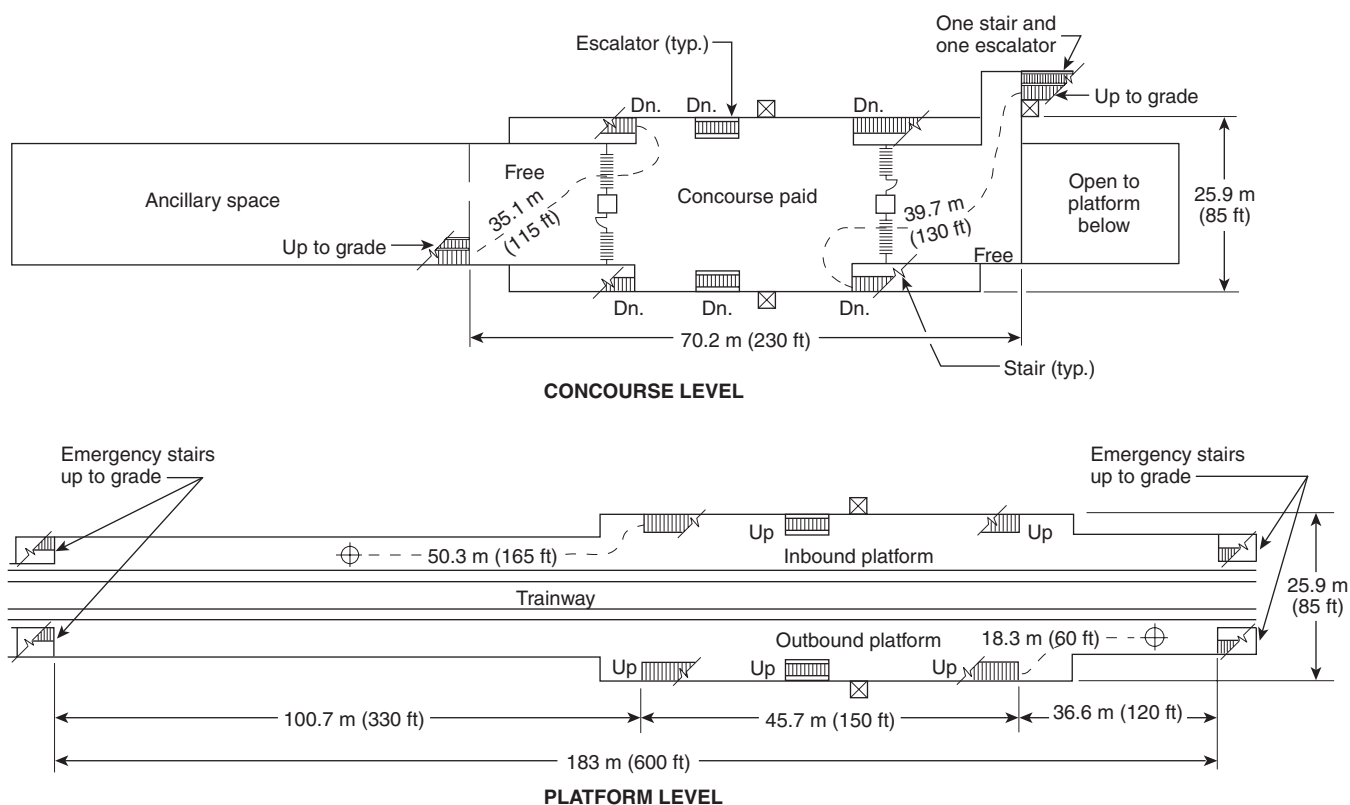
FIGURE C.1.4 Side-Platform Station.
