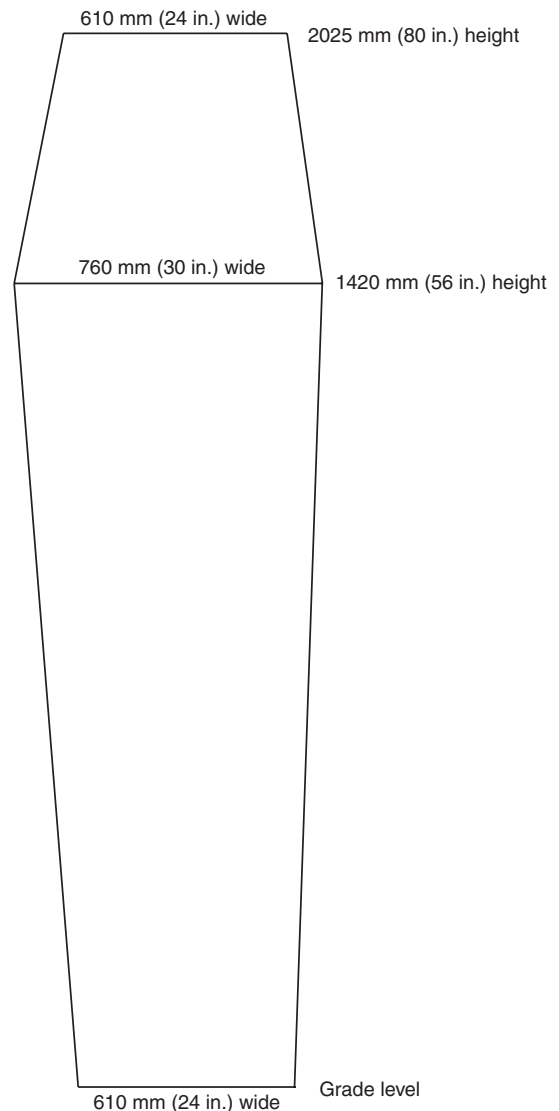
FIGURE A.6.2.1.9 Unobstructed Clear Width for Trainway Walkway.
