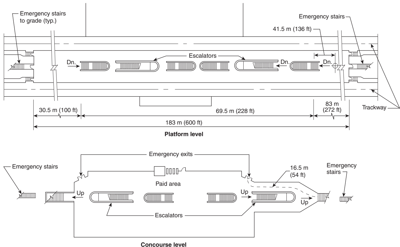
FIGURE C.1.3 Center-Platform Station.
