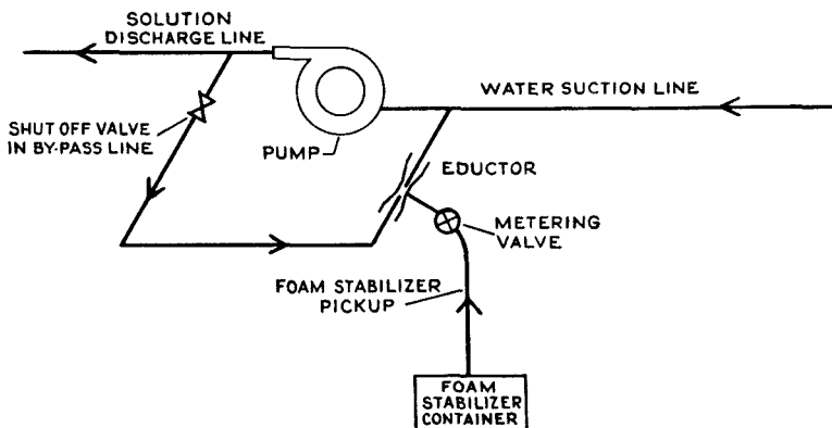
Fig. A-11-55.22. Around-the-Pump Proportioner.
