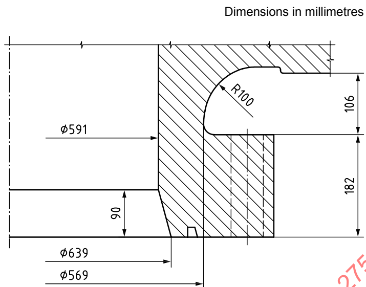
Figure B.4 — Valve design, example B.4.3
