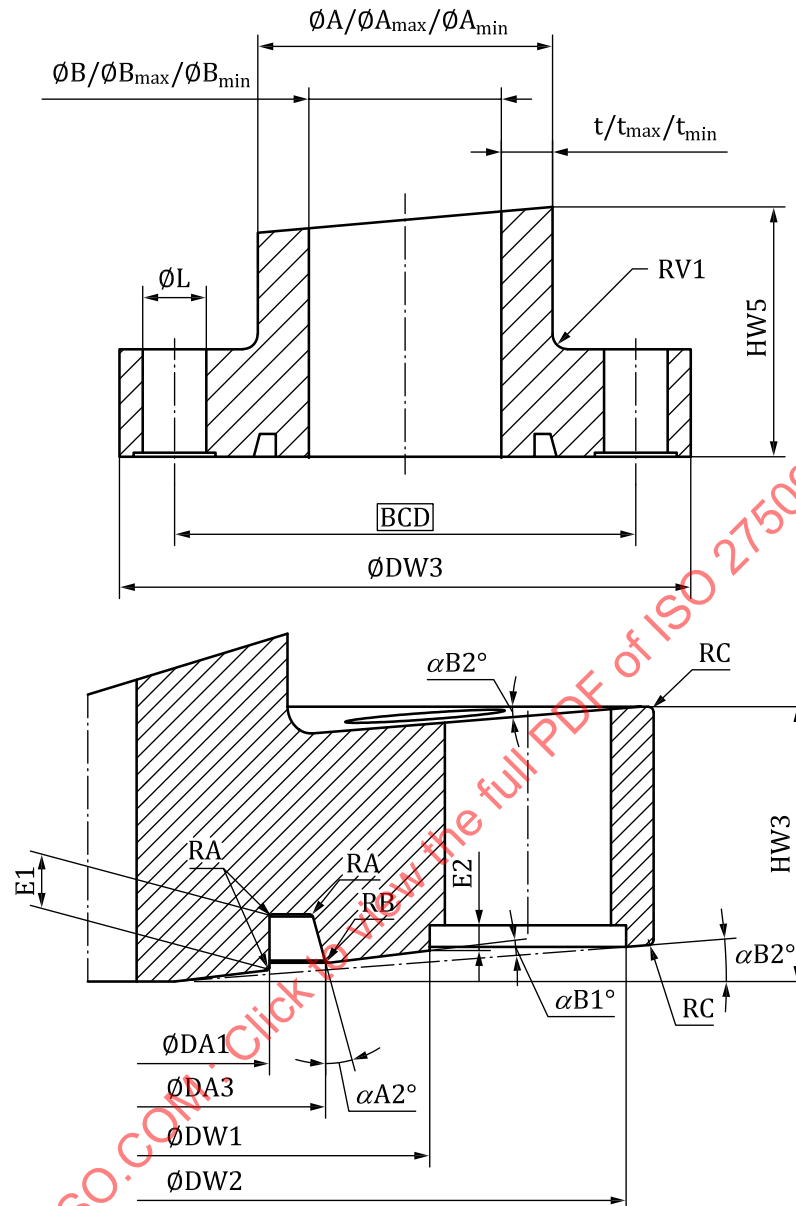
Figure 4 — Nomenclatures for integral flanges
