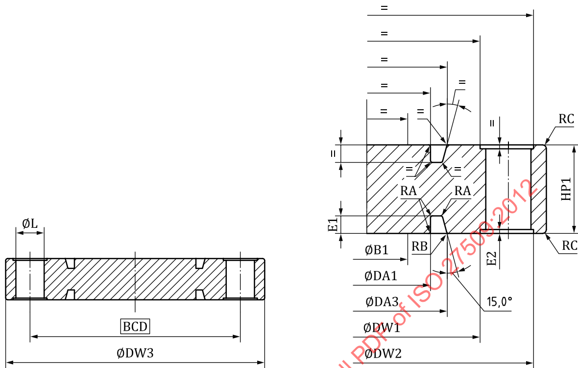
Figure 7 — Nomenclatures for paddle blank (PB) flanges
