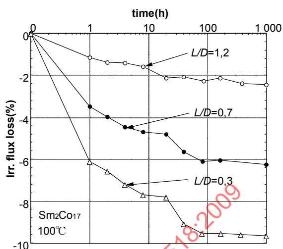
Figure 13 – Time dependence of irreversible flux loss for Sm 2 Co 17 magnets with various L/Ds (Material 2) [24]
