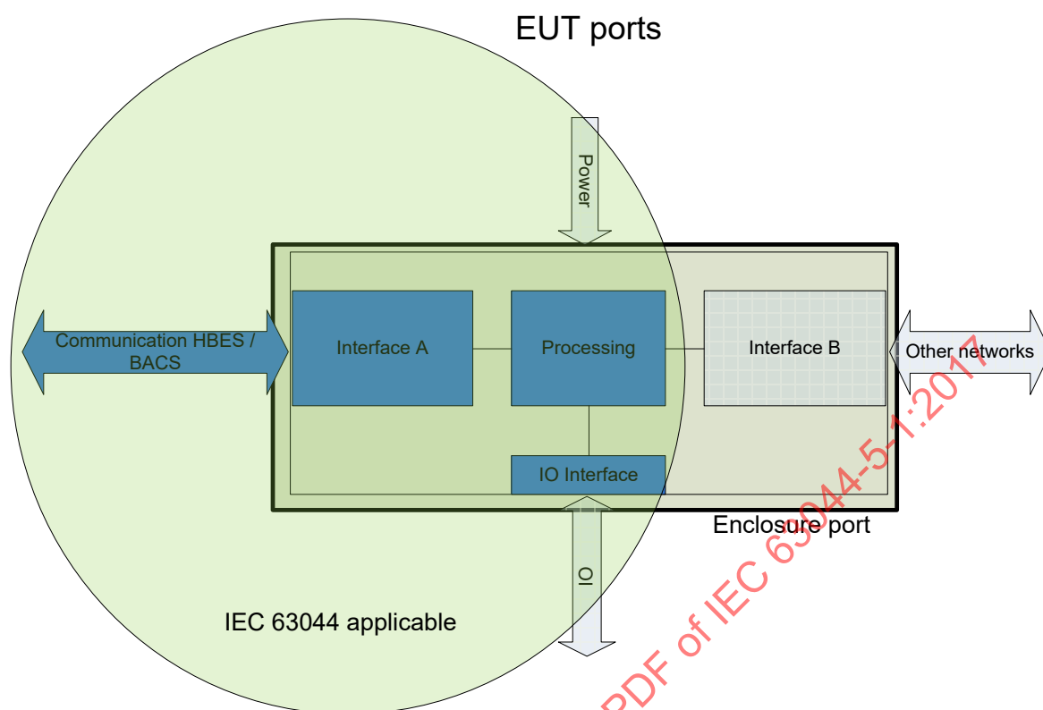
Figure 1 – EUT ports
