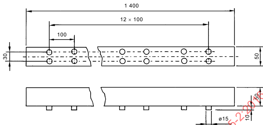
Figure 20 – Carpet hold-downs and guides
