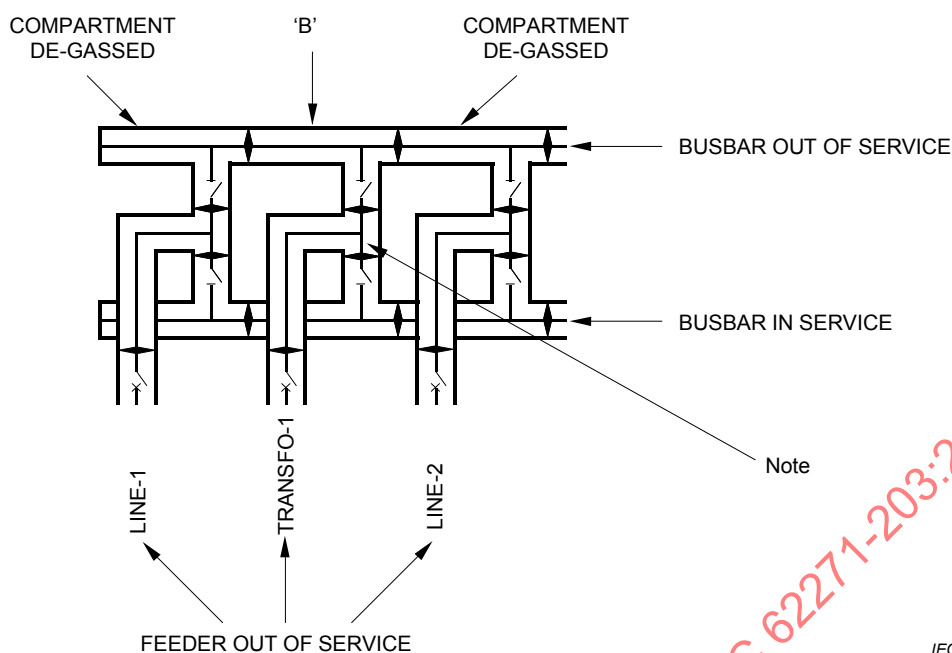
Figure F.2 – Impact of GIS partitioning on service continuity
