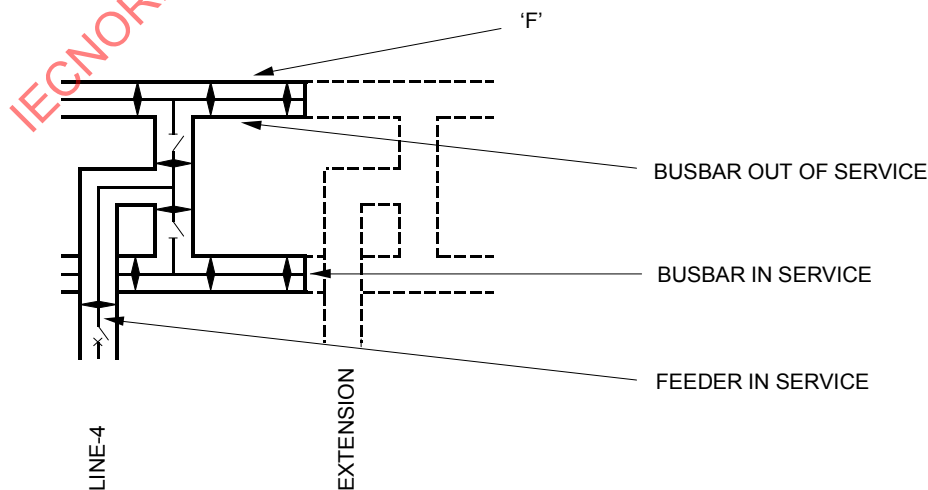
Figure F.7 – Extension
