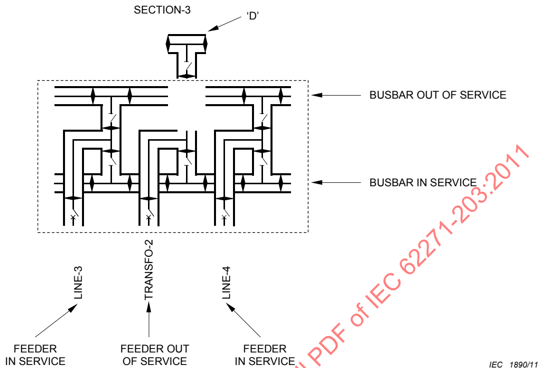
Figure F.6 – Removal of busbar disconnector in SECTION-3
