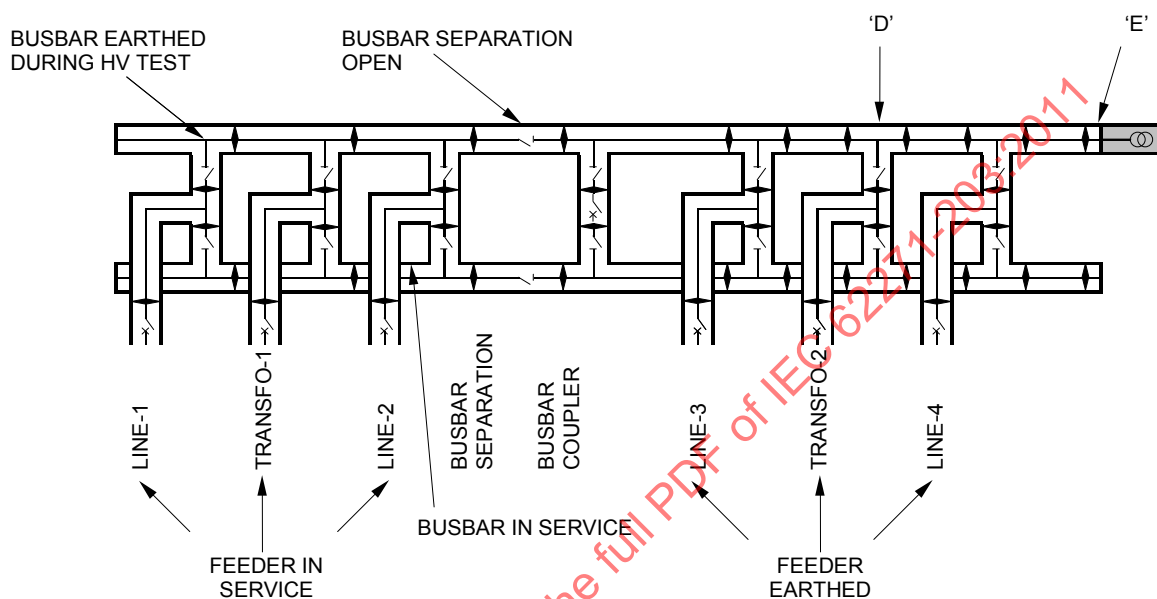
Figure F.8 – On-site dielectric test
