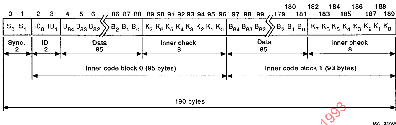
Figure 34 – Sync block format for NTSC and PAL-M
