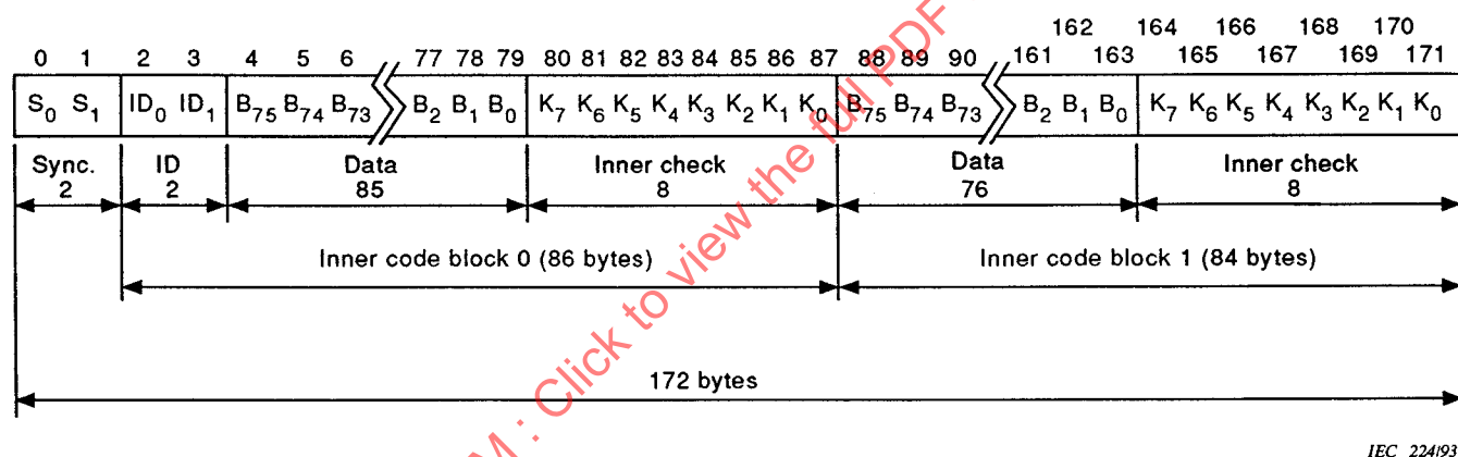
Figure 35 – Sync block format for PAL
