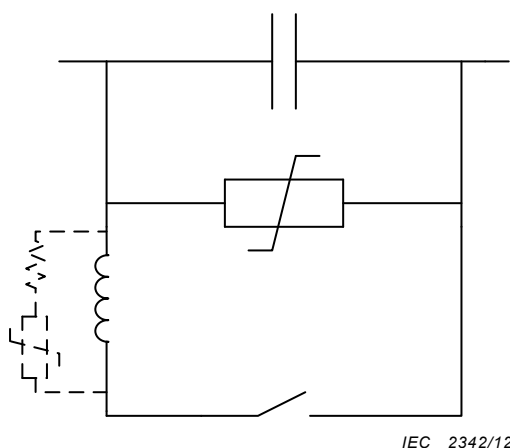
Figure 6 – Conventional location in the bypass branch
