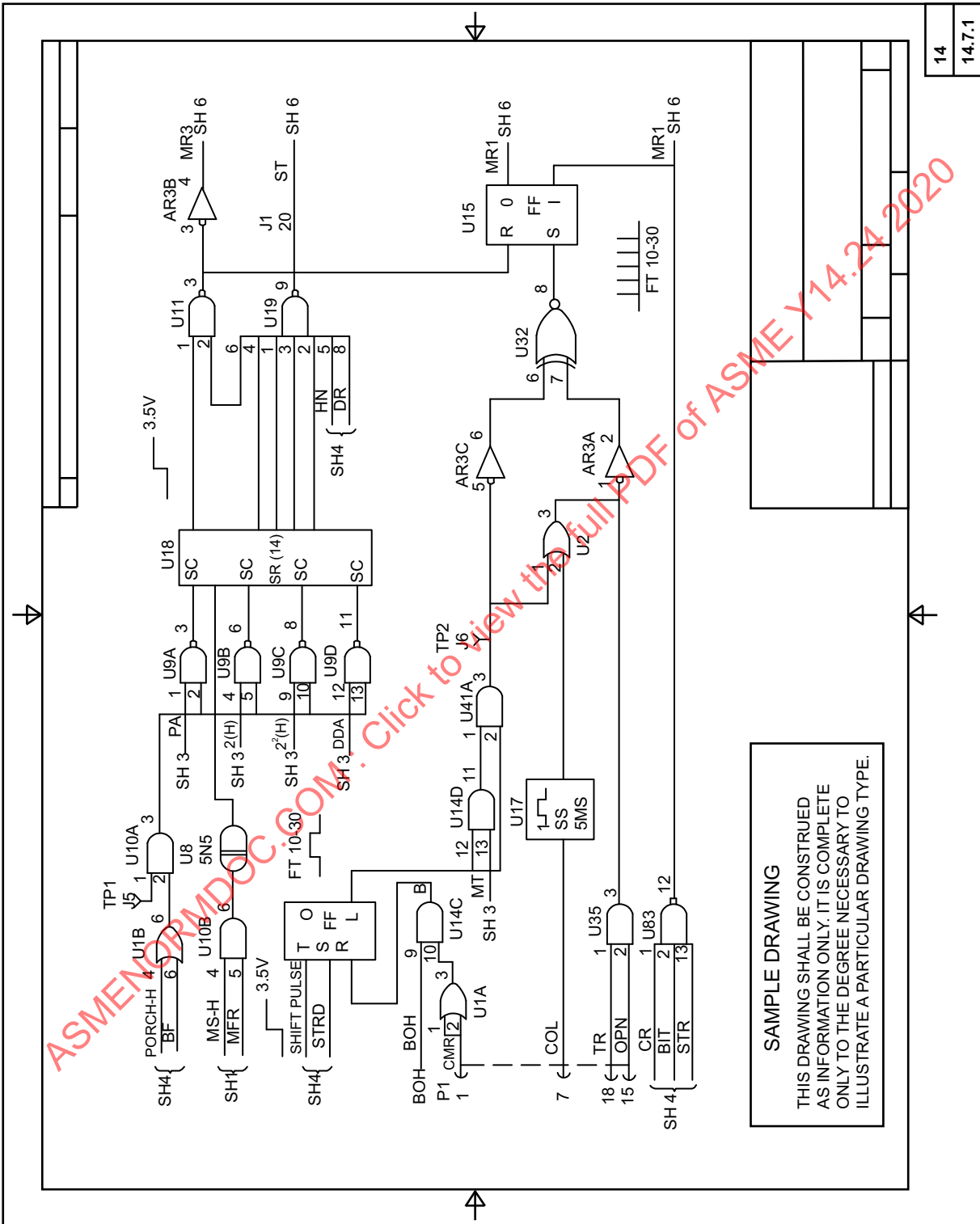
Figure 14.7.1-1 Logic Circuit Diagram
