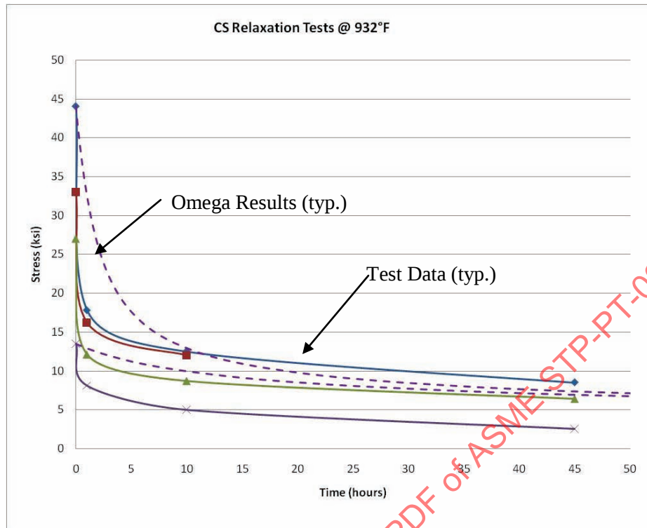
Figure 20 – Uniaxial Carbon Steel Omega Relaxation Results at 932°F
