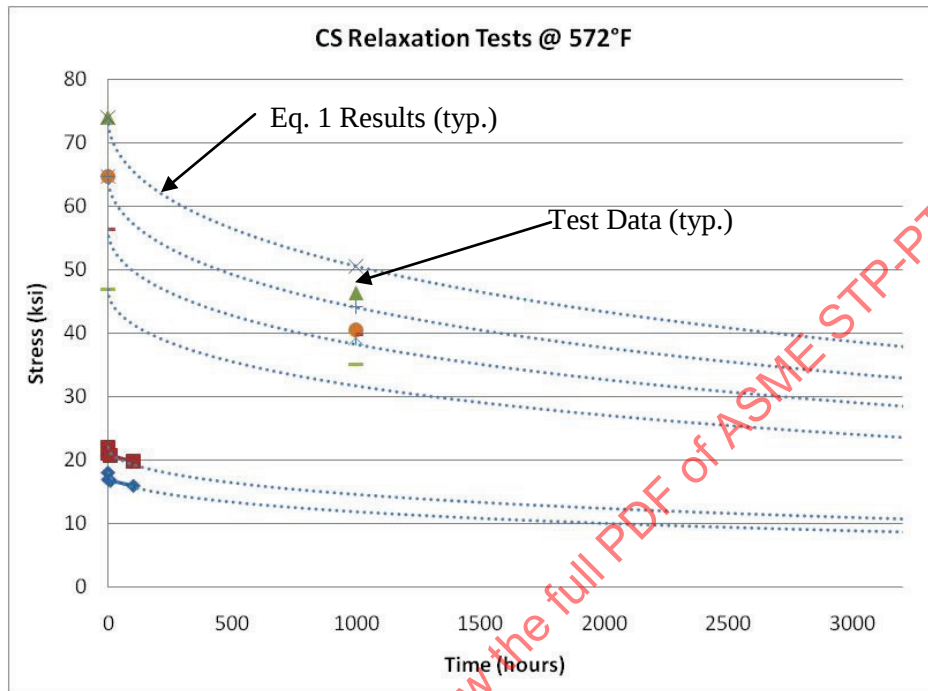
Figure 21 – Equation (1) Carbon Steel Relaxation Results at 572°F
