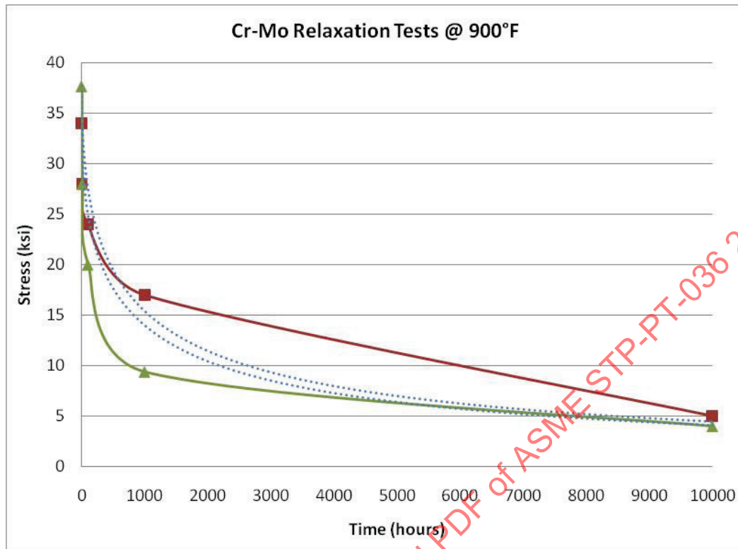
Figure 31 – Equation (1) CrMo Relaxation Results at 900°F
