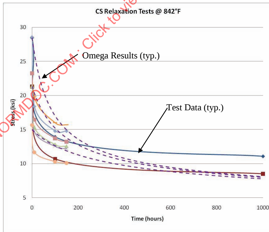
Figure 19 – Uniaxial Carbon Steel Omega Relaxation Results at 842°F
