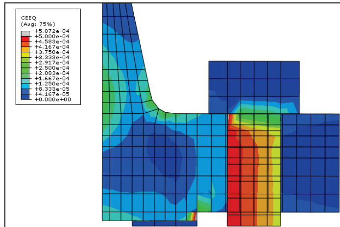
Figure 40 – NPS 3, cl. 150 Creep Strain @ 217 hrs
