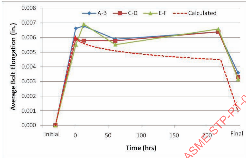
Figure 57 – NPS 2, cl.900 Bolt Deformation Results
