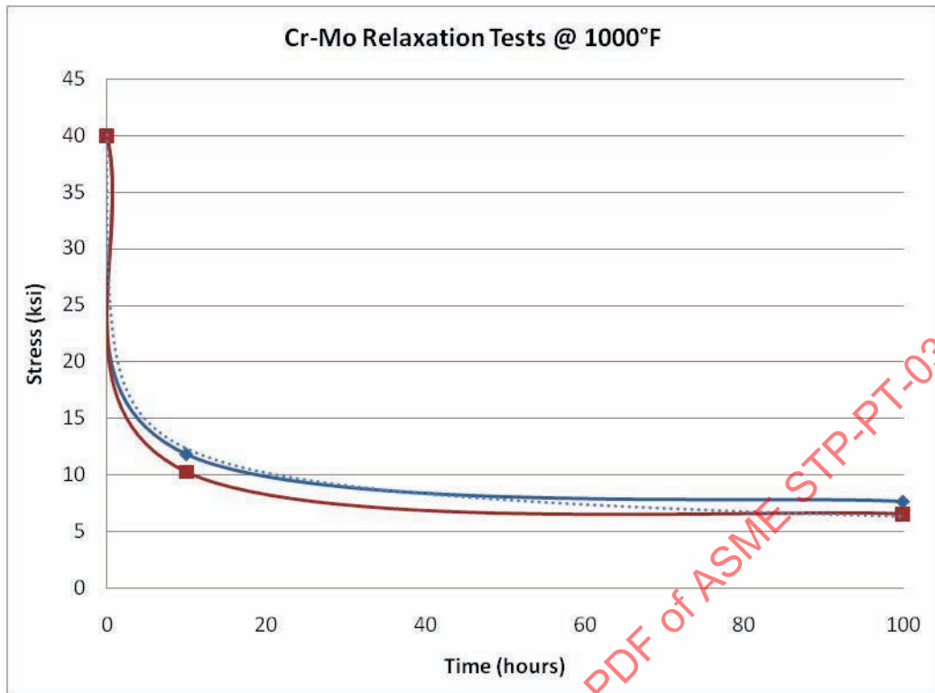
Figure 33 – Equation (1) CrMo Relaxation Results at 1000°F
