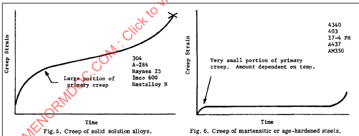
Figure 13 – Creep Characteristics of Different Materials from Cooper, et. al. [14], Fig. 5 to Fig.7, page 133
