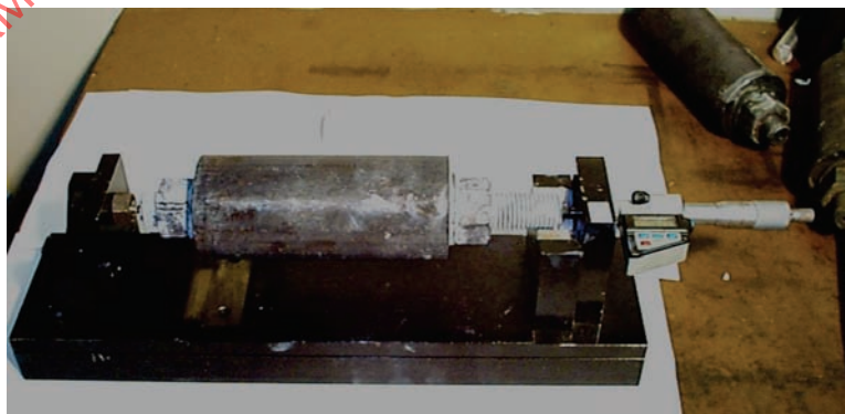
Figure 50 – Length Measurement Arrangement
