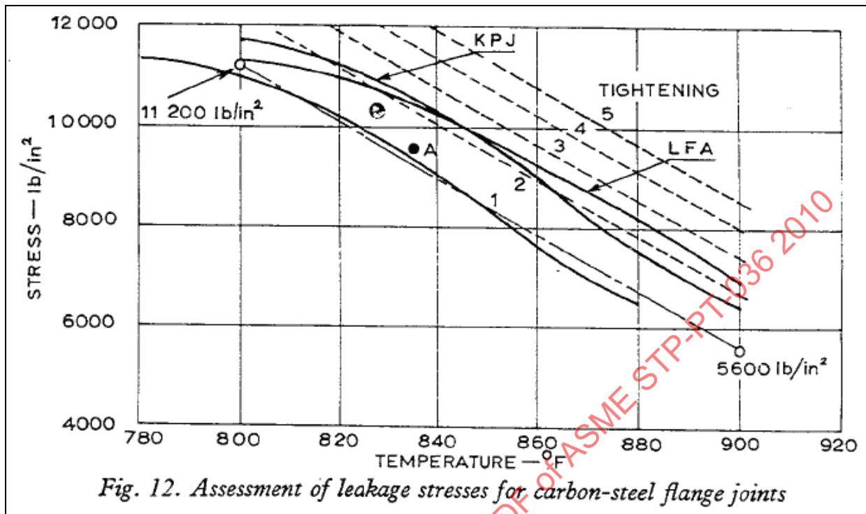
Figure 11 – Comparison of Flange Test Results vs. Creep Tests from Bernhard [13], Fig. 12, page 122
