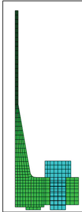
Figure 43 – NPS 6, cl. 150 FEA Model
