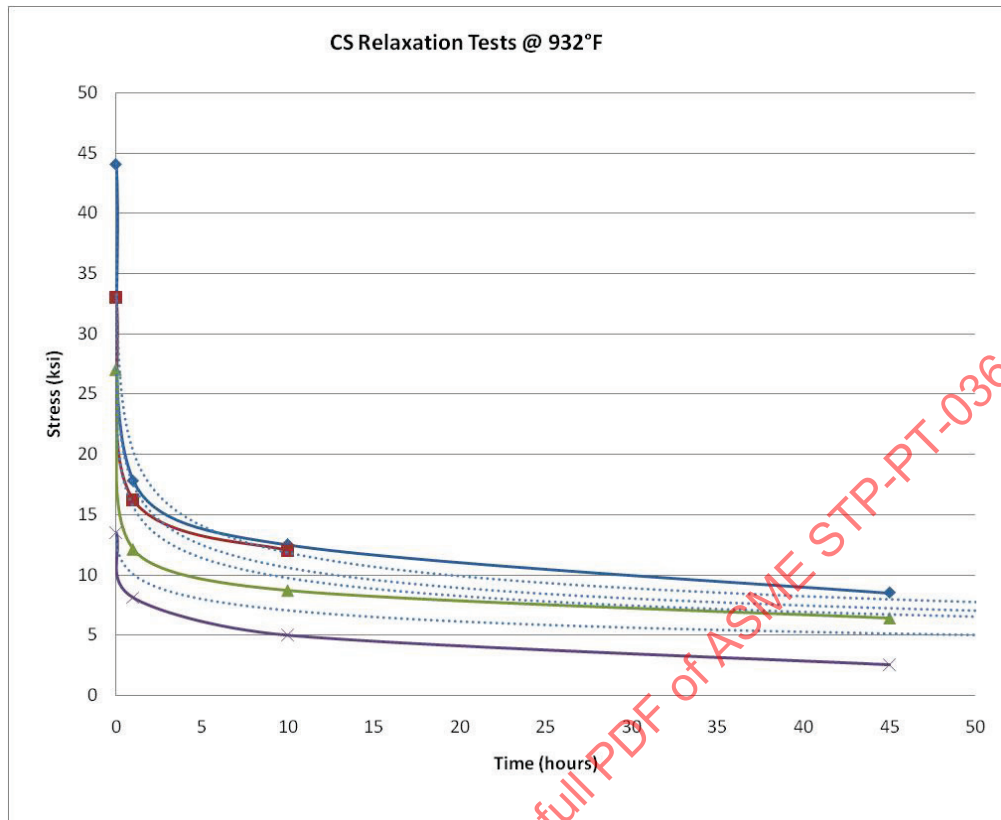
Figure 23 – Equation (1) Carbon Steel Relaxation Results at 932°F
