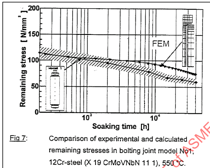
Figure 15 – FEA Bolt Load Relaxation Results from Maile, et. al. [18], Fig. 7, page 156
