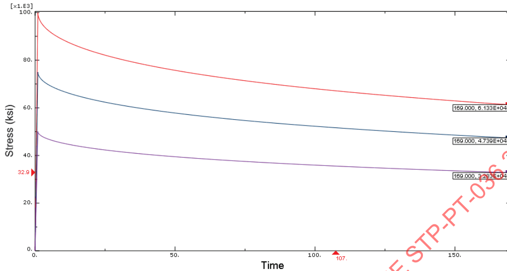
Figure 36 – Bolt/Cylinder Full FEA Model Bolt Stress vs. Time Results
