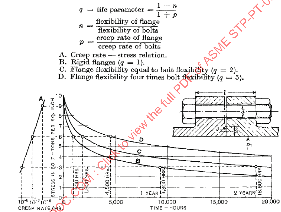
Figure 1 – From Baumann [3], page 1336
