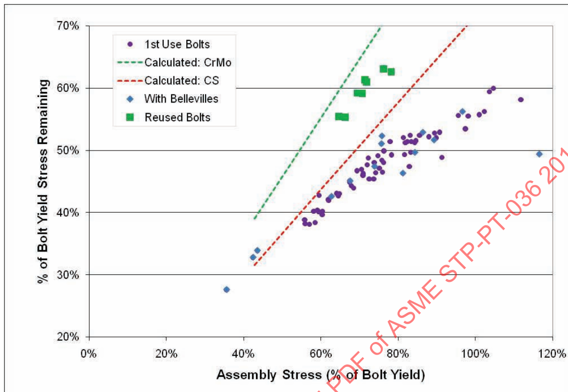
Figure 56 – Bolt Load Relaxation vs. Assembly Load (% of Ambient Bolt Yield Stress)
