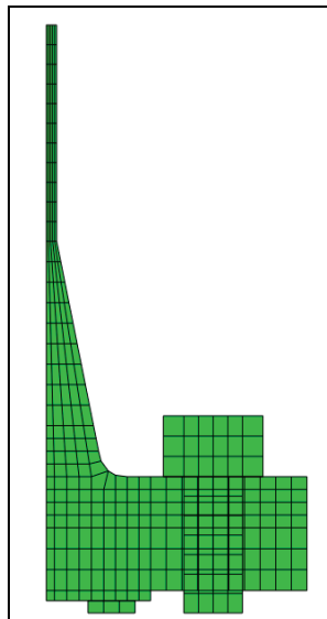
Figure 39 – NPS 3, cl. 150 FEA Model
