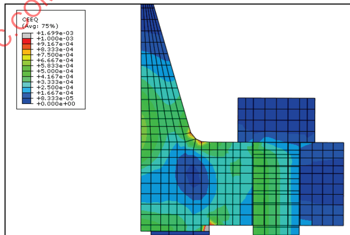
Figure 42 – NPS 3, cl. 300 Creep Strain @ 217hrs
