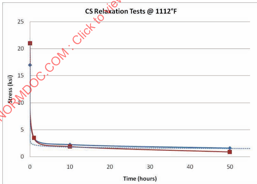
Figure 24 – Equation (1) Carbon Steel Relaxation Results at 1112°F
