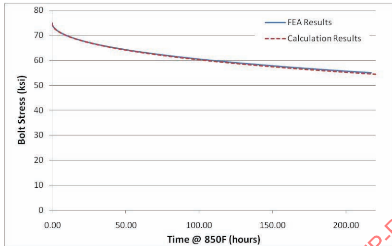
Figure 47 – NPS 6, cl. 150 Bolt Stress vs. Time
