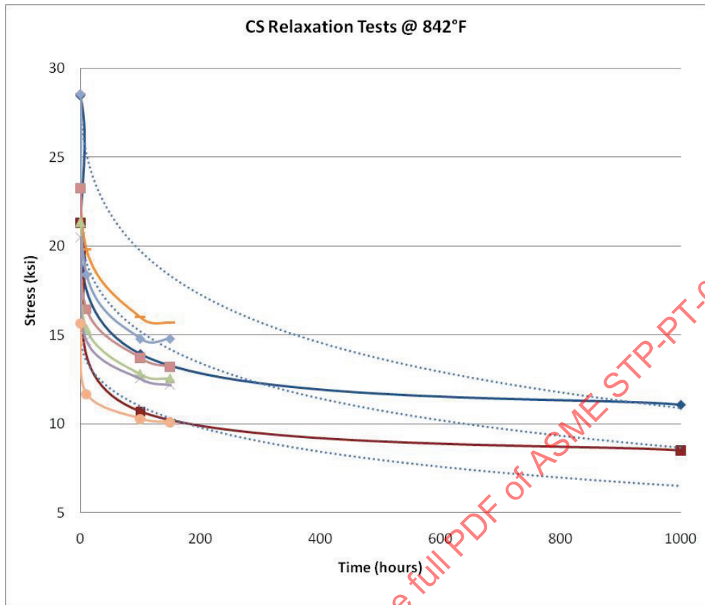
Figure 25 – Equation (1) Carbon Steel Relaxation Results at 842°F
