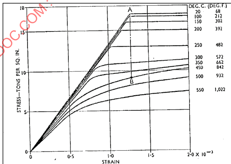
Figure 9 – Carbon Steel Pipe Flange Strength vs. Temperature from Johnson [11], Fig. 28, page 448
