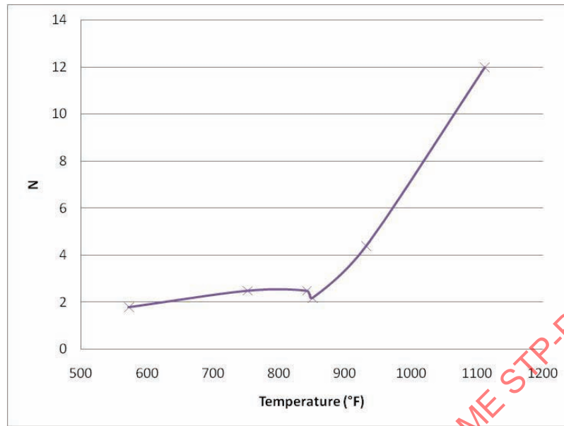
Figure 27 – Equation (1) Carbon Steel “N” vs. Temperature
