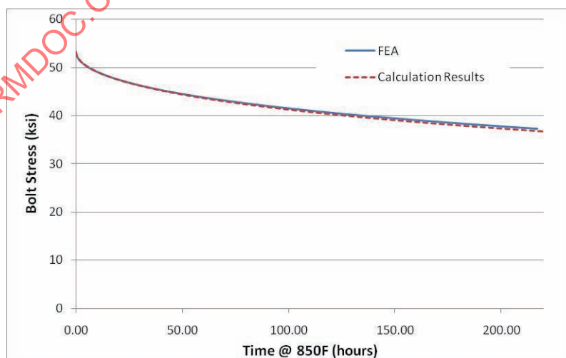
Figure 46 – NPS 3, cl. 300 Bolt Stress vs. Time
