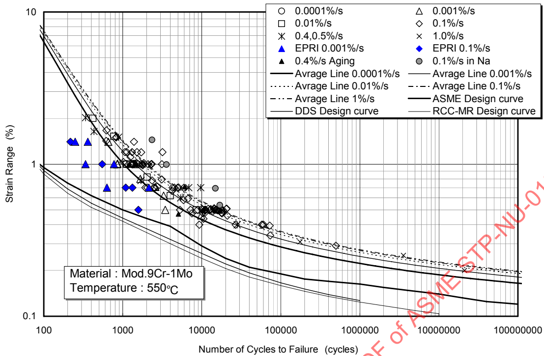
Figure 5 - Fatigue Life: Average Curves and Experimental Values at 550°C
