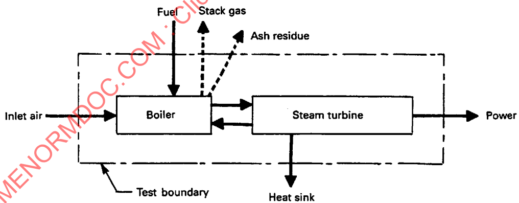
FIG. 3.2 TYPICAL STEAM PLANT TEST BOUNDARY
