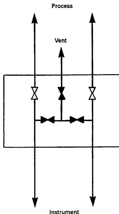
FIG. 4.1 FIVE-WAY MANIFOLD
