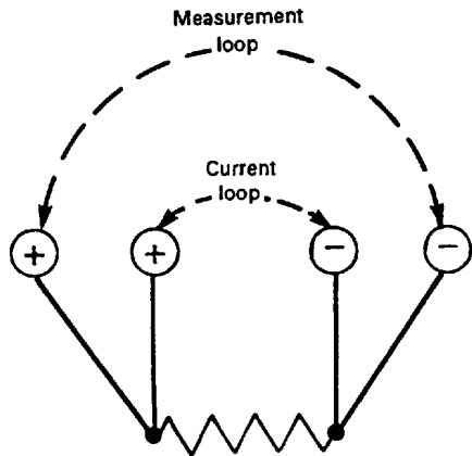
FIG. 4.2 FOUR-WIRE RTDs
