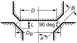
Bevel-Seated Valve
