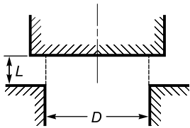
Flat-Seated Valve
