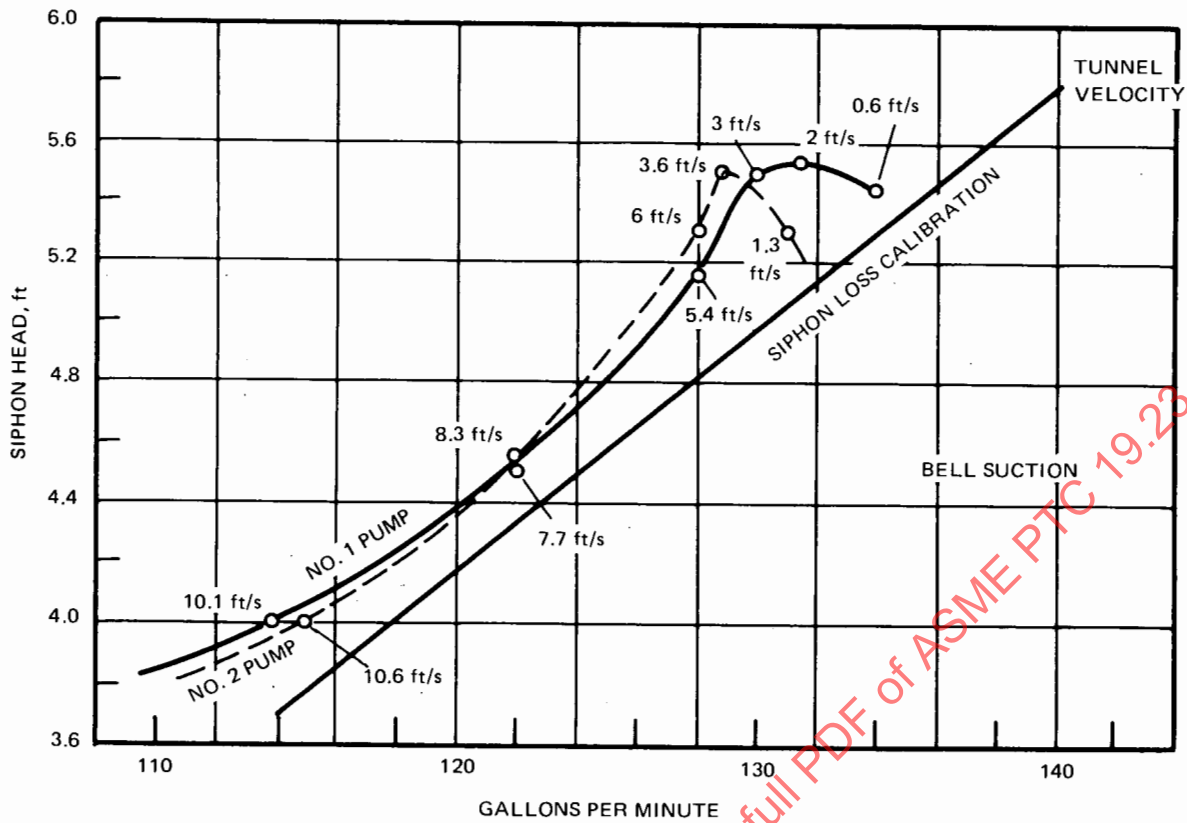
EX. 2-4 SIPHON LOSS WITH BELL SUCTION
