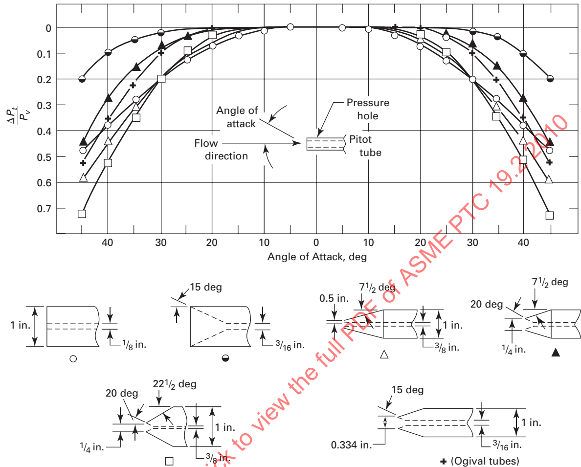
Fig. 5-2.1.1-2 Variation of Total Pressure Indication With Angle of Attack and Geometry for Pitot Tubes
