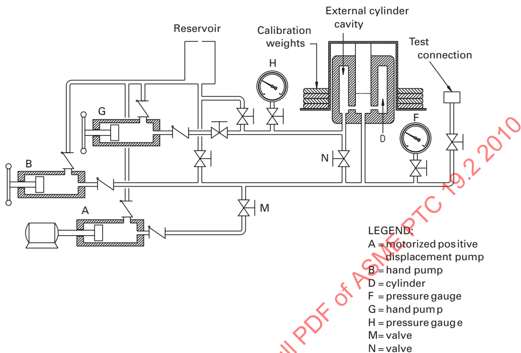
Fig. A-1.3-1 Controlled-Clearance Cylinder Piston Gauge
