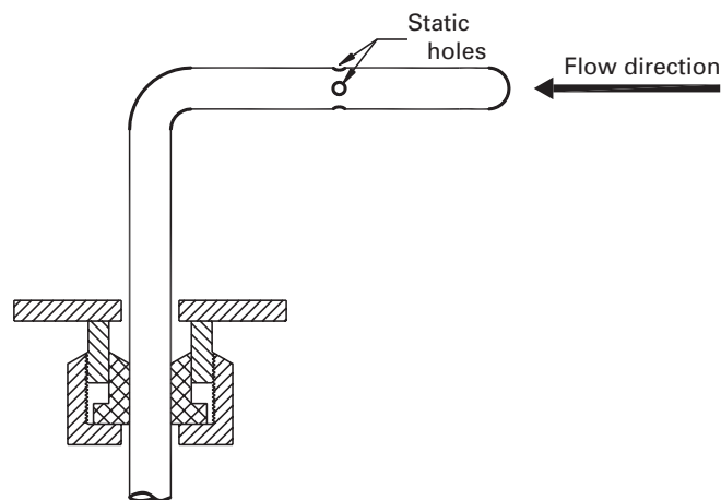
Fig. 5-2.2.1-1 Static Tube
