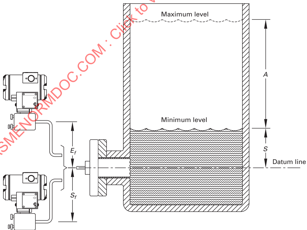
Fig. 3-2.1.2.1-3 Open-Tank Installation With Remote-Seal Type of Transmitter
