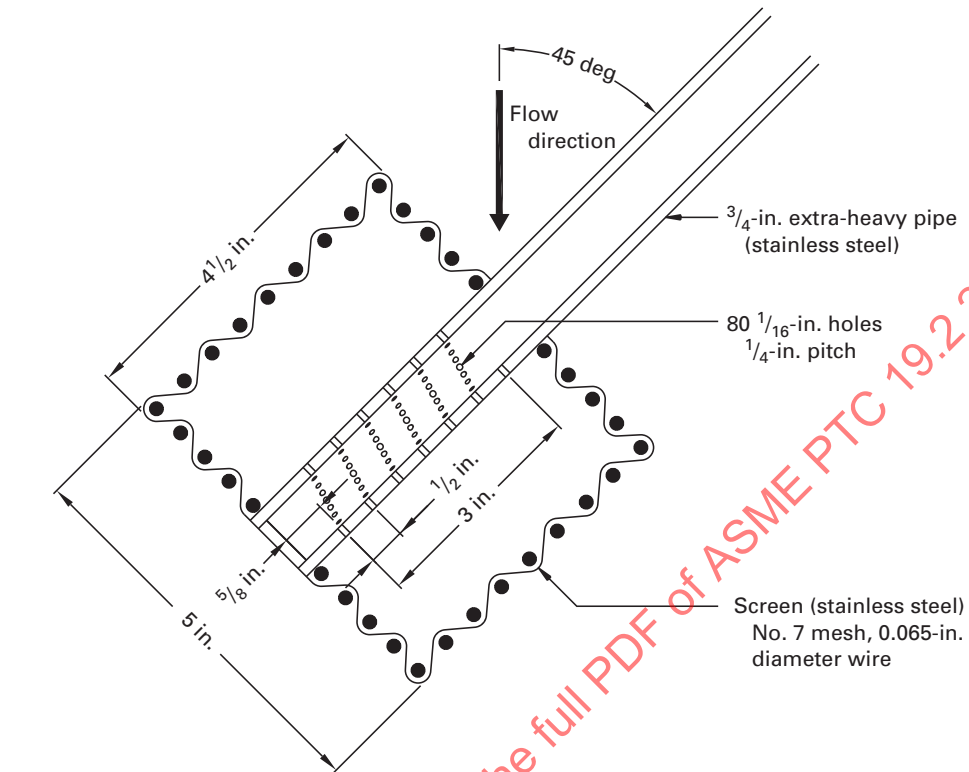
Fig. 5-2.2.3-2 Alternate Basket Probe
