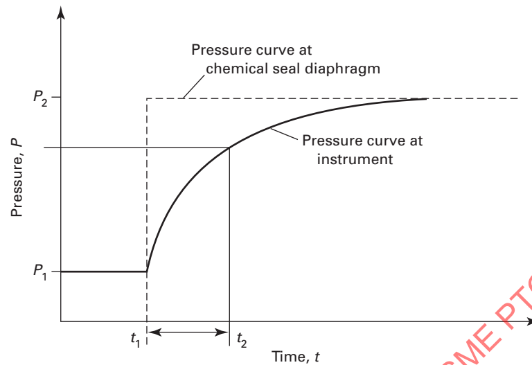
Fig. 5-4.9-1 Response Time
