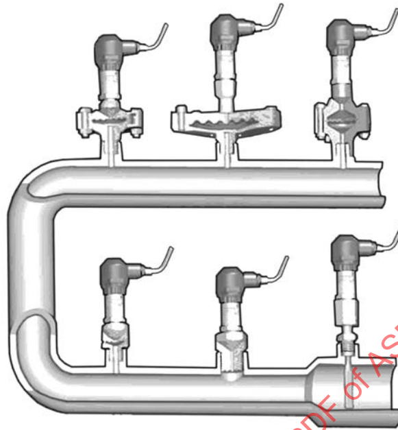
Fig. 5-4.3-4 Threaded Diaphragm Seal
