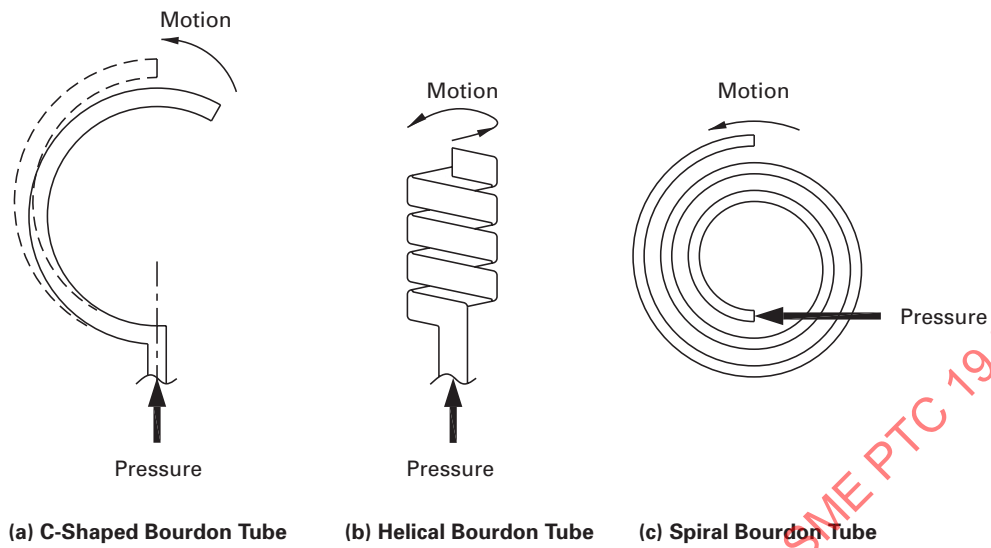
Fig. 3-3.1.1-2 Bourdon Tubes
