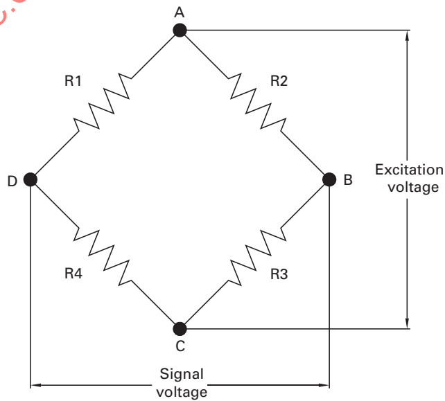
Fig. 3-1.2.1-1 Wheatstone Bridge
