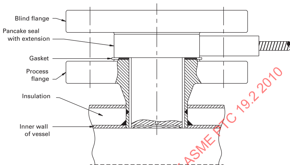
Fig. 5-4.3-11 Pancake Extension
