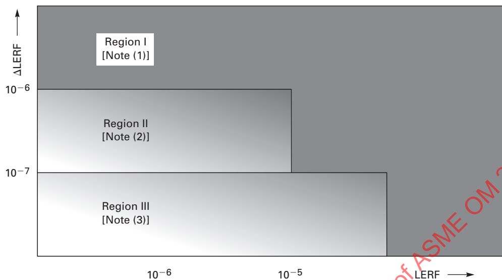
Fig. L-2100-2 Acceptance Guidelines for LERF (From RG 1.174)
