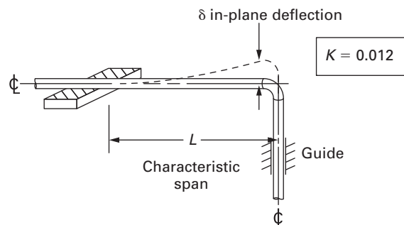
Fig. 6 Cantilever Span/Elbow Guided Span in-Plane Deflection Measurement
