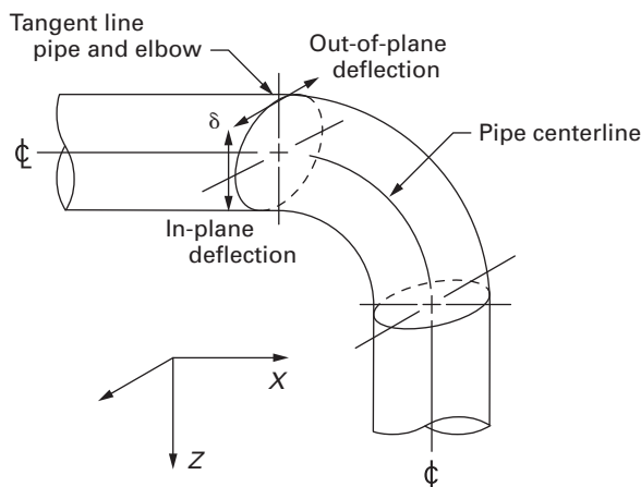
Fig. 2 Deflection Measurement at the Intersection of Pipe and Elbow
