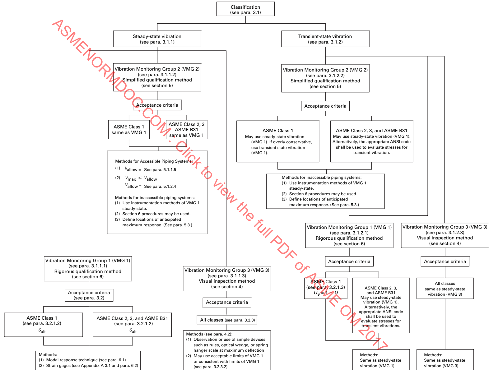
Fig. F-1 Flowchart — Outline of Vibration Qualification of Piping Systems
