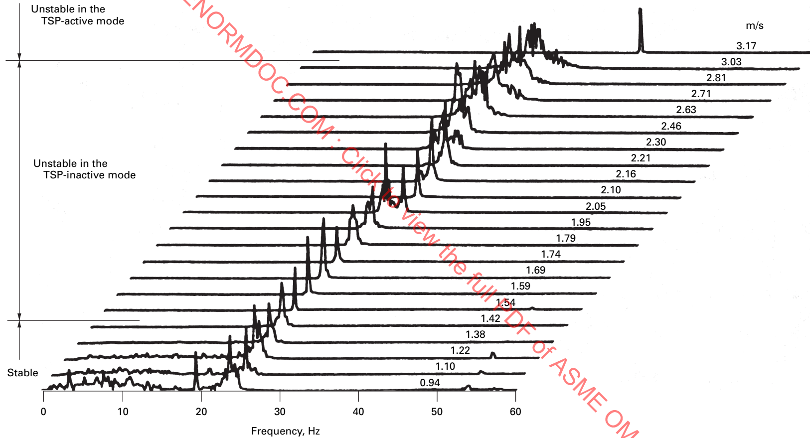
Fig. E-12 Frequency Spectra of Tube Displacement at Location "A" (Diametral Gap of 1.27 mm)
