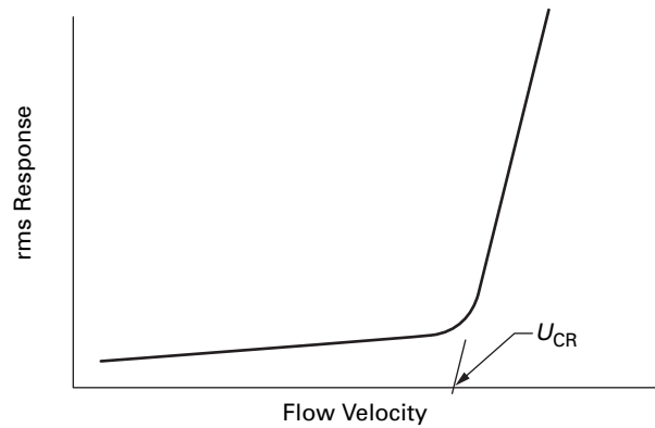
Fig. E-3 Root Mean Square (rms) Tube Response Versus Flow Velocity
