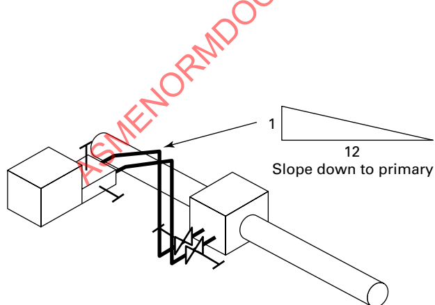
FIG. C3 GAS SERVICE, SECONDARY ABOVE PRIMARY
