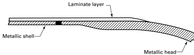
Figure 10-201-2 Laminate Termination
