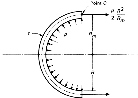
Figure AC-100.3
