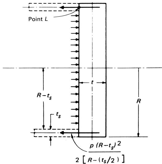
Figure AC-100.5
