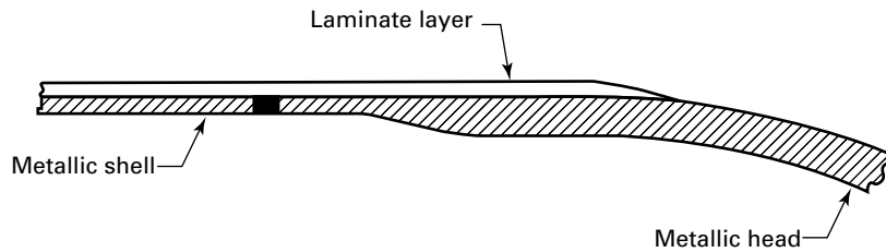
Figure 10-201-2 Laminate Termination
