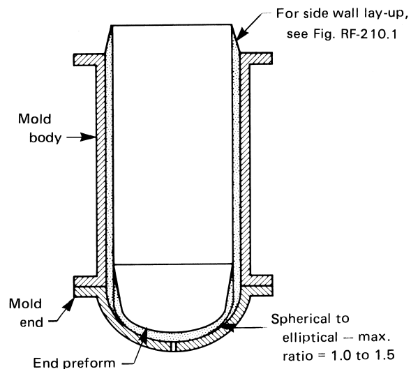
Figure RF-210.2 Head or End Preform for Cylindrical Vessel
