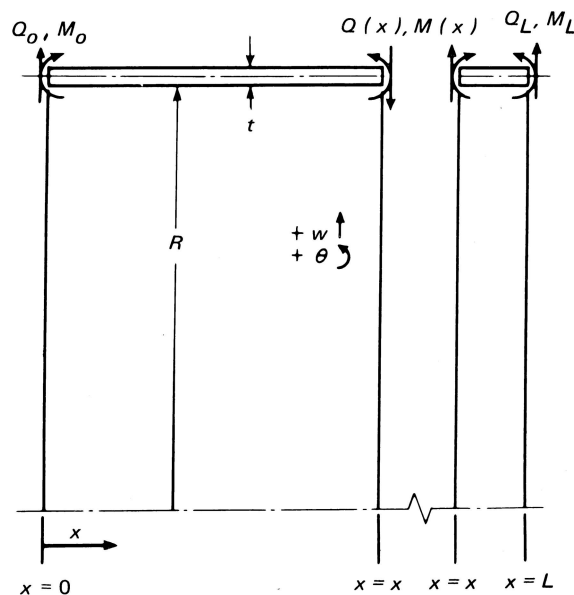
Figure AC-200 Symbols and Sign Convention
