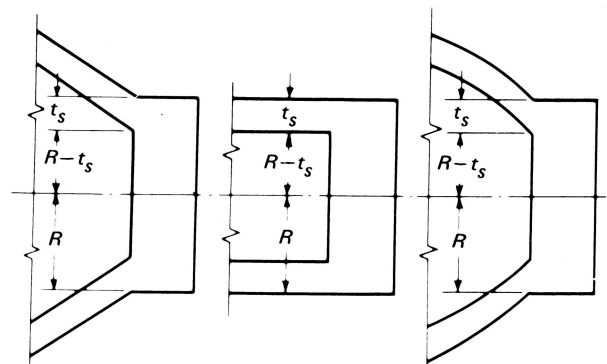
Figure AC-430
