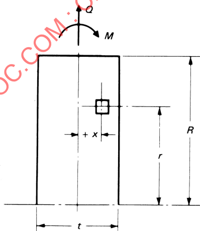
Figure AC-422
