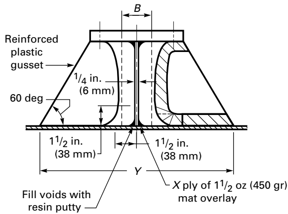
Figure RD-620.4(a) Plate-Type Gussets
