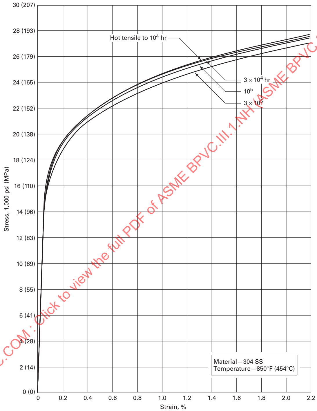
Figure NH-T-1800-A-2 Average Isochronous Stress–Strain Curves
