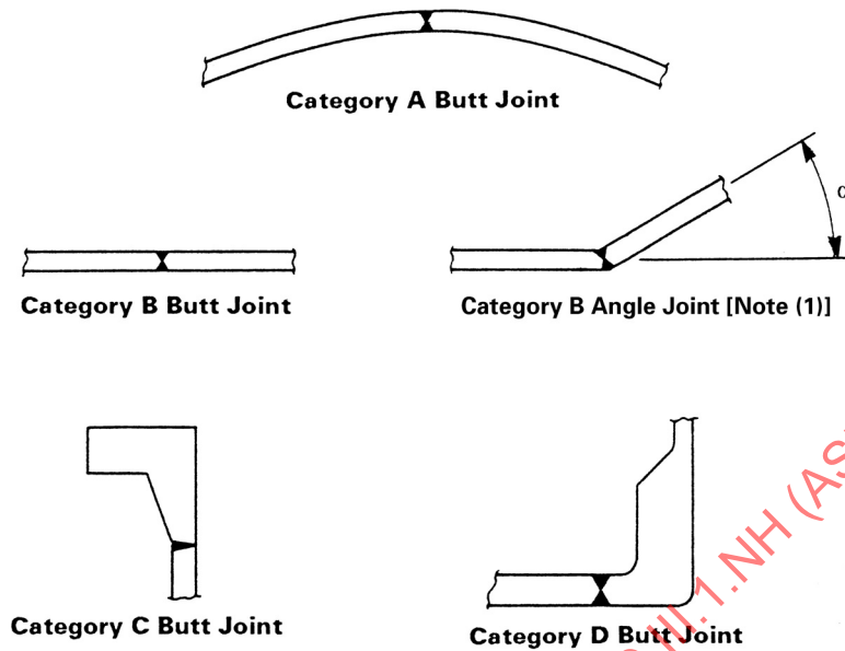
Figure NH-3352-1 Typical Butt Joints
