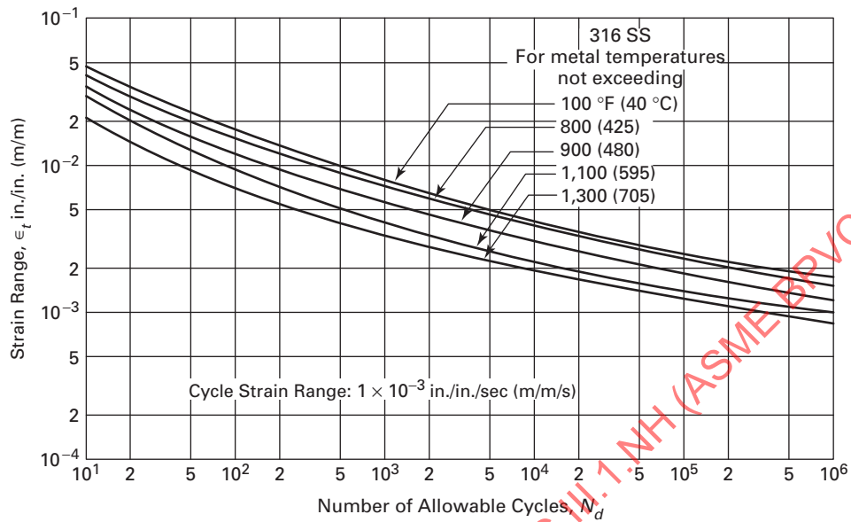
Figure NH-T-1420-1B Design Fatigue Strain Range, \epsilon_t , for 316 SS
