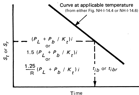
Figure NH-3224-2 Use-Fractions for Membrane Plus Bending Stress
