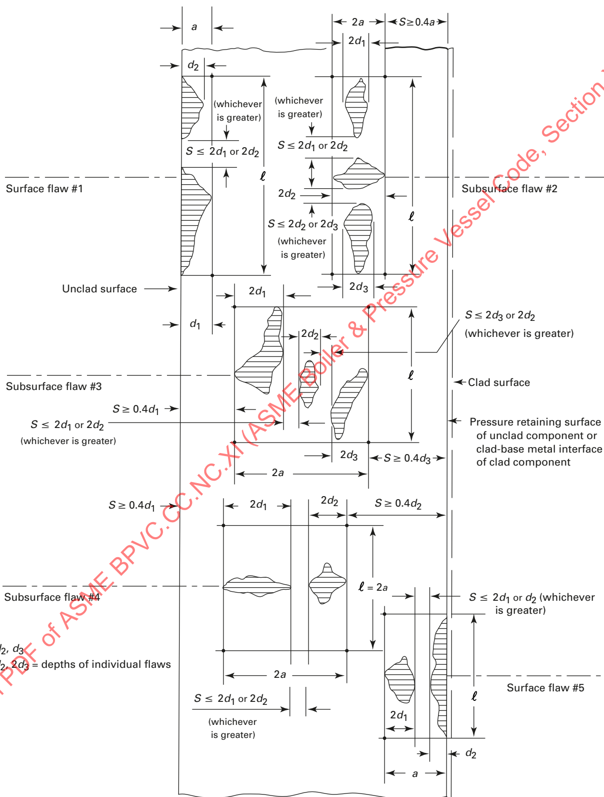
Figure 2 Multiple Planar Flaws Oriented in Plane Normal to Pressure Retaining Surface
