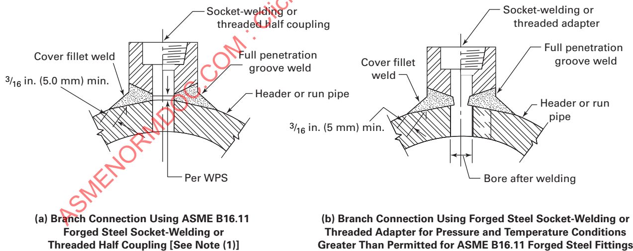
Fig. 127.4.8(F) Typical Full Penetration Weld Branch Connections for NPS 3 and Smaller Half Couplings or Adapters
