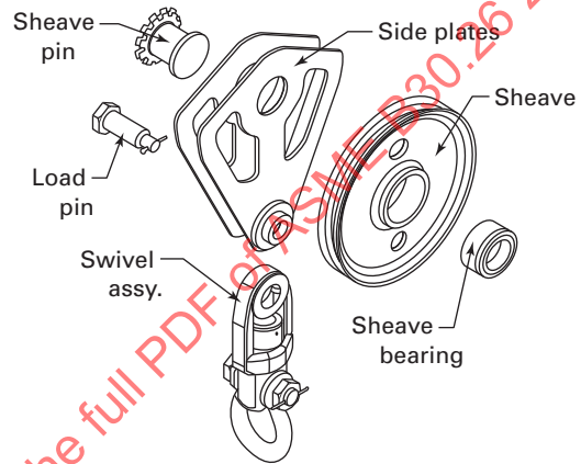
Rolling Block
