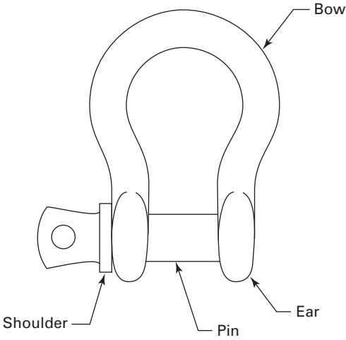
Fig. 26-1.9.4-1 Typical Shackle Components
