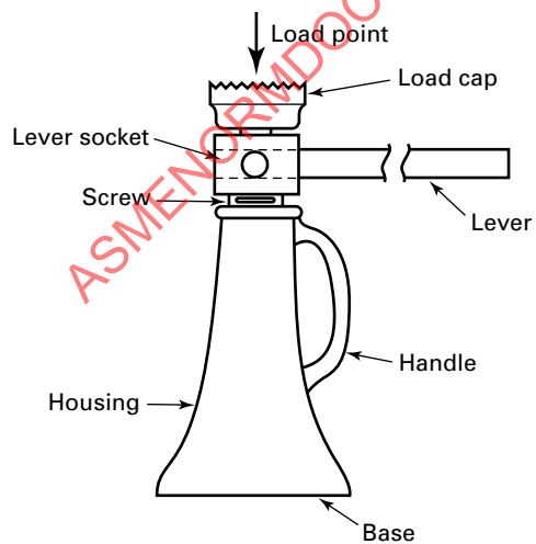
Figure 1-1.1.1-2 Screw Jack
