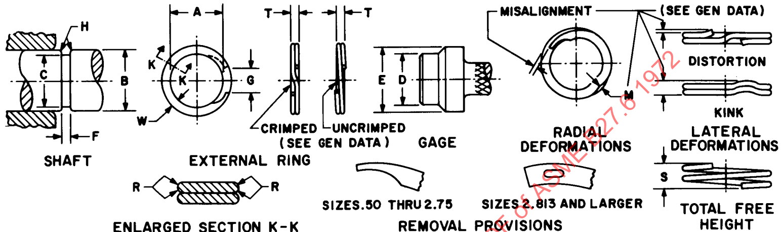
ENLARGED SECTION K-K Table 1. Dimensions of Type 2A01 Light Duty External Retaining Rings, Grooves, and Gages (Continued)
