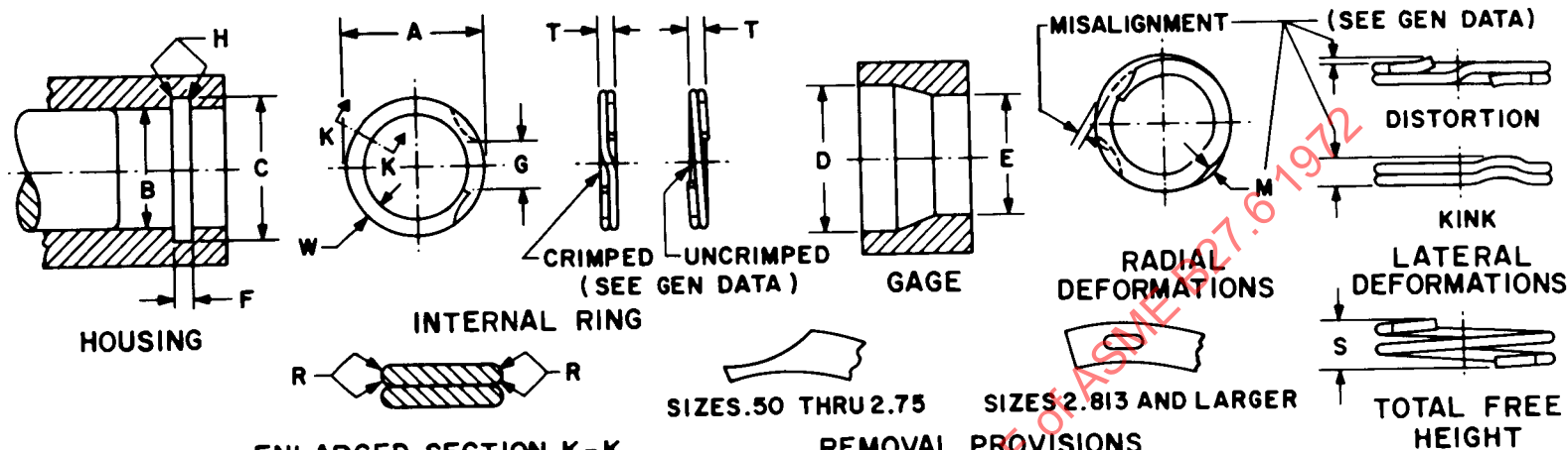
ENLARGED SECTION K-K
